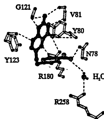
Figure 4. The observed crystallographic model of pteric acid (PTA) binding in the active site of RTA
