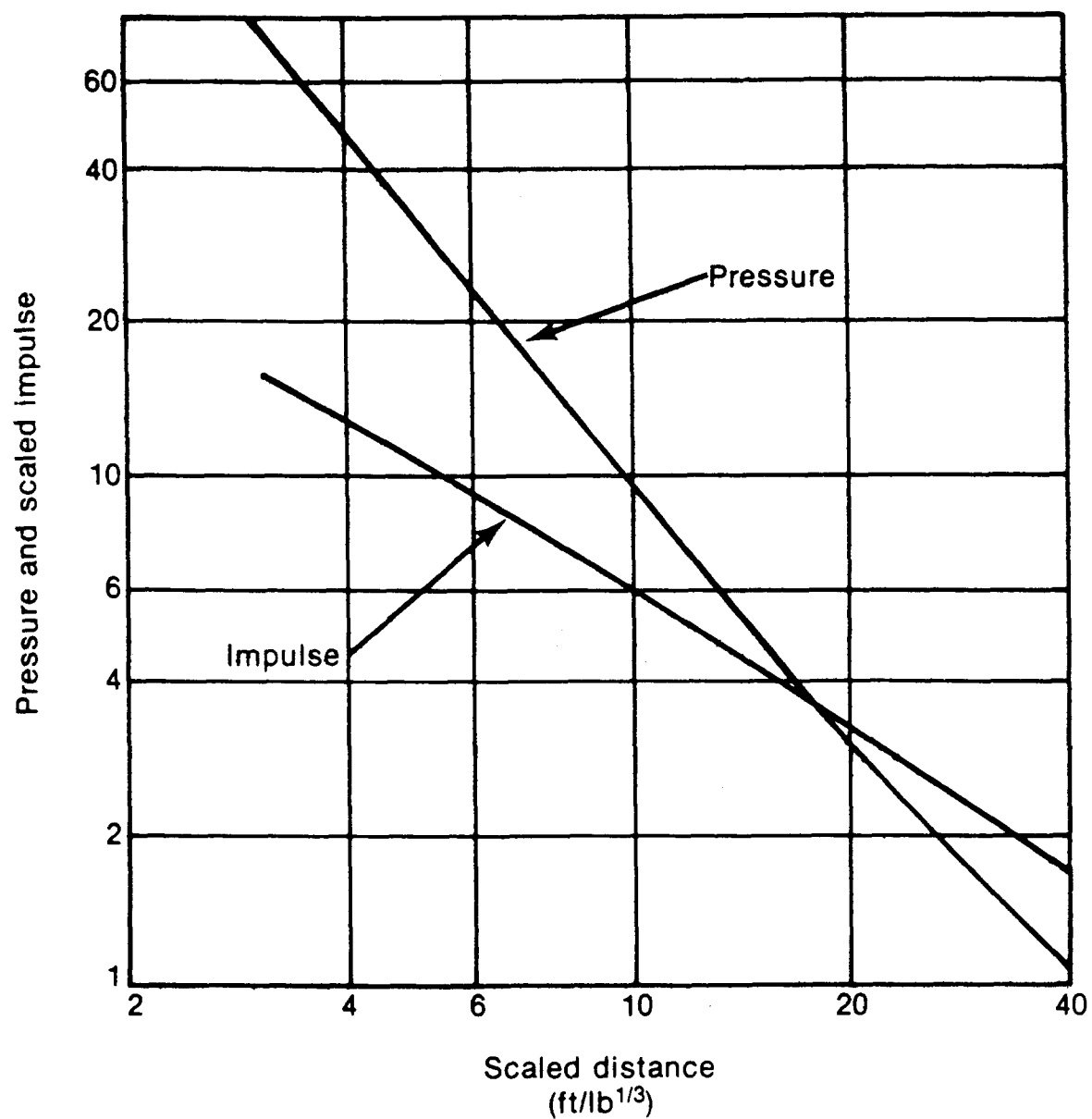
Figure 140. Peak Pressure and Scaled Positive Impulse Versus Scaled Distance for the Combined Weights for AL/KClO 4 .
