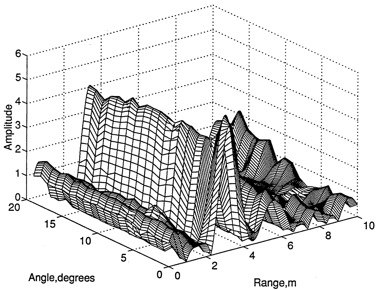
Range Profiles of Airplane
