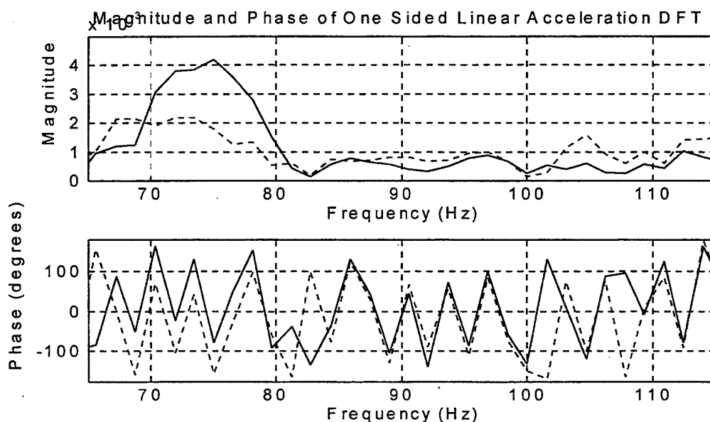
Figure 5.22. Plot of the magnitude and phase (degrees) of the one-sided linear acceleration DFT of accelerometers located at 6 and 7 on "rocky" in the X-direction from 65 to 115 Hz; for extracting azimuth jitter; data from firing eight (cf8_1_5s).
