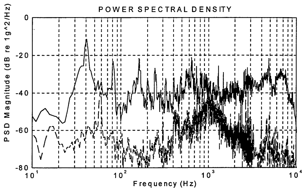
Figure 5.18. Plot of the PSD (solid line) and pre-firing noise (dashed line) for location seven in the X- direction; from test firing one (cf8_1_5s) data. The g rms in the 20 to 2000 Hz band is 0.862 g rms.
