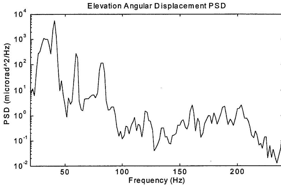
Figure 5.28. Plot of the elevation displacement PSD 20 to 240 Hz after correcting for coherence.
