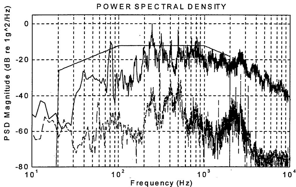
Figure 5.8. Plot of the PSD (solid line), pre-firing noise (dashed line), and specification for location three in the Z-direction; from test firing one (cf1_1_5s) data. The acceleration in the 20 to 2000 Hz frequency band is 6.116 g rms.
