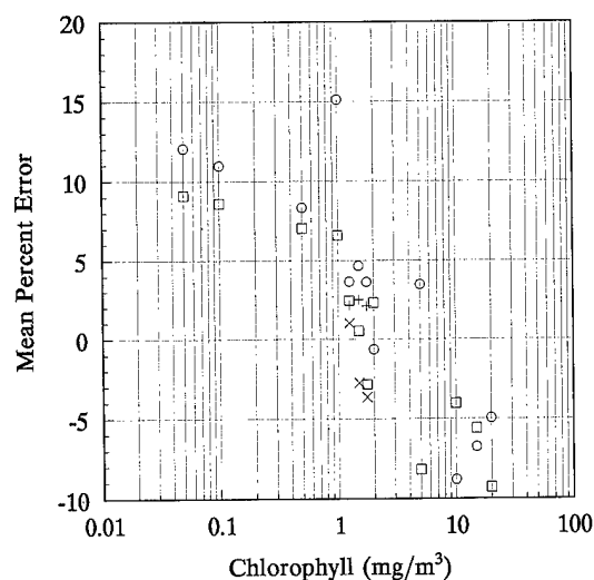
Figure 4. Mean percent error in backscattering retrieval as a function of chlorophyll for air mass 2 ( 60^\circ solar angle); symbols as in Figure 3.
