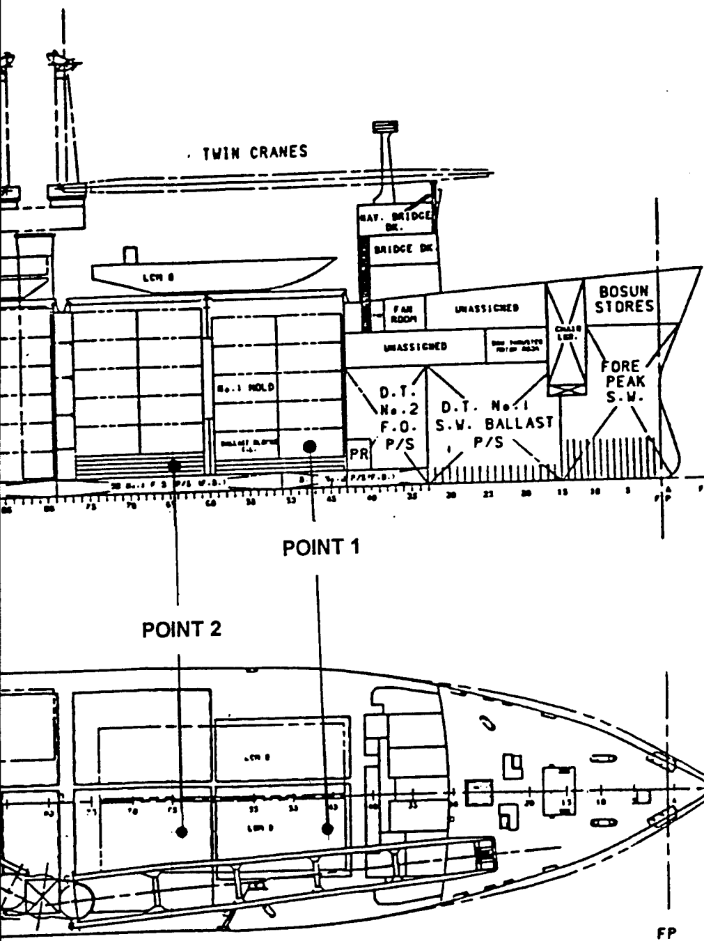
Fig. 2. T-ACS 4 sketches to illustrate the selected cargo locations. (a) T-ACS 4 inboard profile sketch showing longitudinal and vertical point locations. (b) T-ACS 4 plan view sketch showing lateral and longitudinal point locations.
