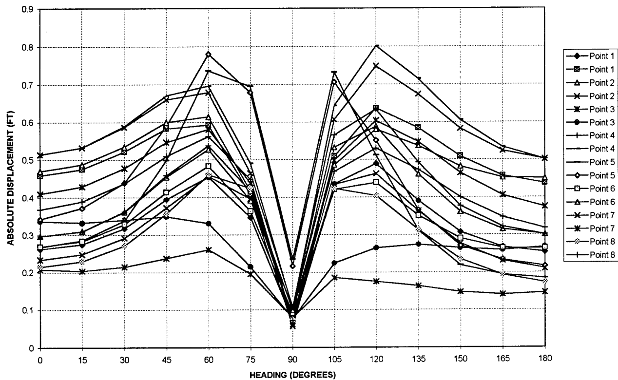
Fig. B.7. Absolute longitudinal displacement vs. heading for Bretschneider spectra of 8 and 9 second modal periods. Significant wave height 6.17 ft. Free floating case.
