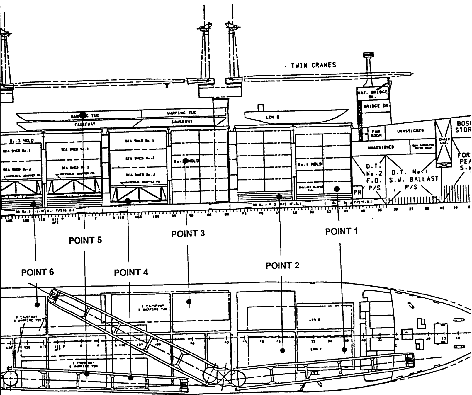
Fig. 2. T-ACS 4 sketches to illustrate the selected cargo locations. (a) T-ACS 4 inboard profile sketch showing longitudinal and vertical point locations. (b) T-ACS 4 view sketch showing lateral and longitudinal point locations.
