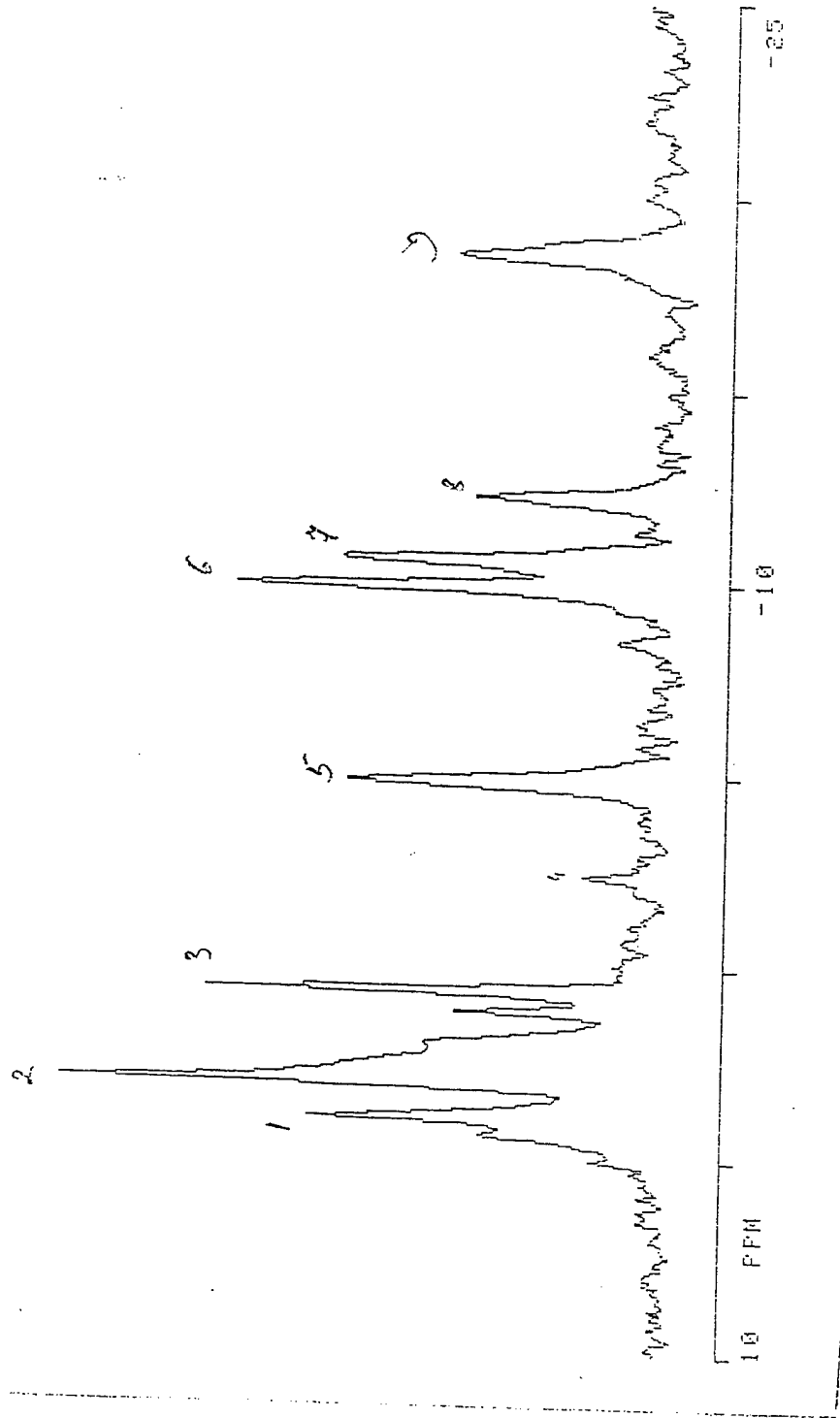
Fig. 3. 51P NMR spectrum of perfused MCF7 cells grown in matrigel threads in the NMR tube.
