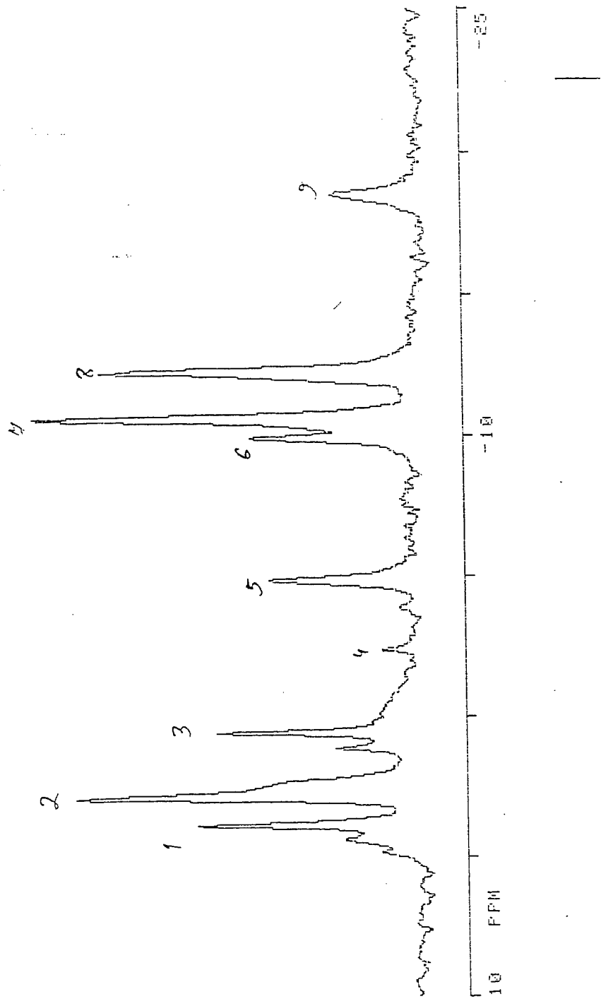
Fig. 6. 31P NMR spectrum of perfused LCC2 cells grown in matrigel threads in the NMR tube.
