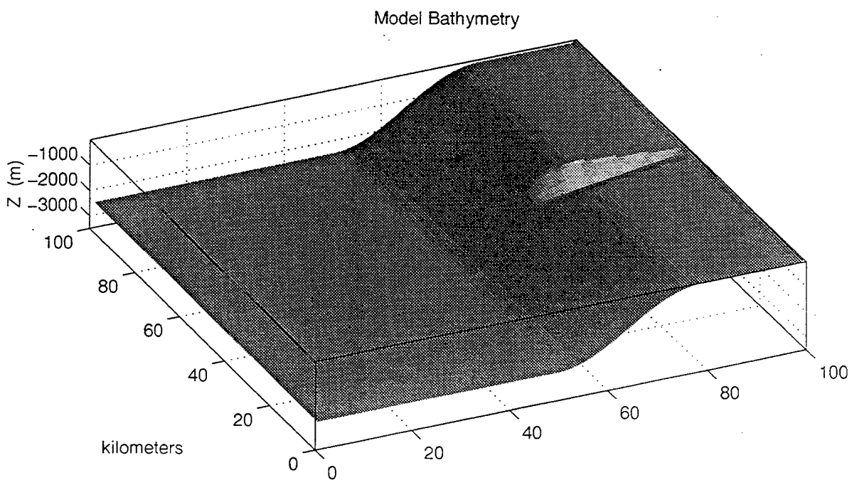
Figure 33. Monterey Bay Bathymetry and a Sample Model Bathymetry. Observed Monterey Bay bathymetry and model bathymetry that incorporates a relatively narrow shelf, a steep ( 7^\circ ) continental slope, a deep basin, and a canyon head lying close to shore.
