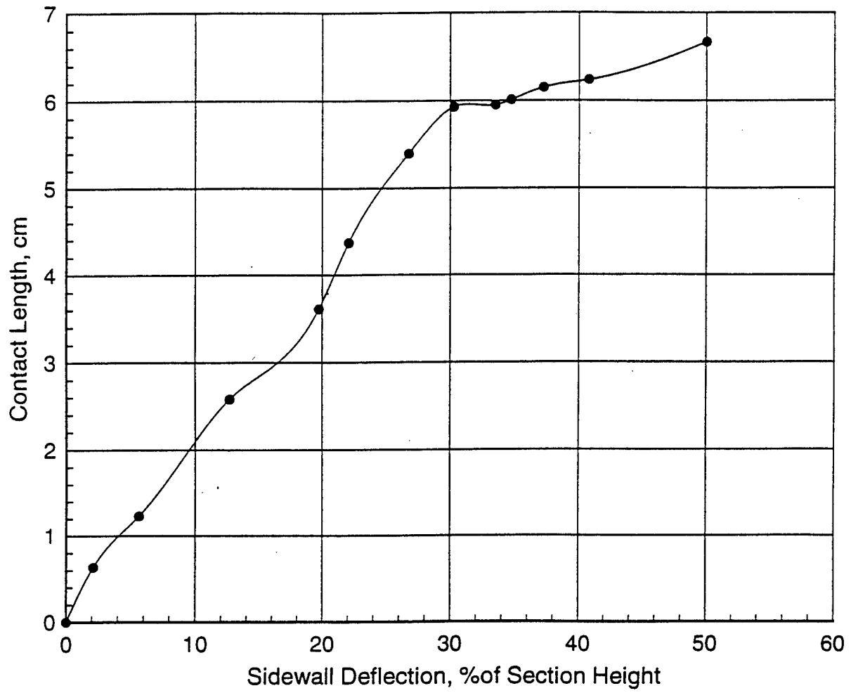
Figure 6.2.13 Variation of Ground Contact Length With Sidewall Deflections
