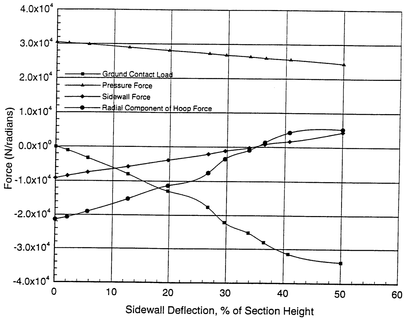
Figure 6.2.4 Various Forces Acting on the Axisymmetric Model of the Tire
