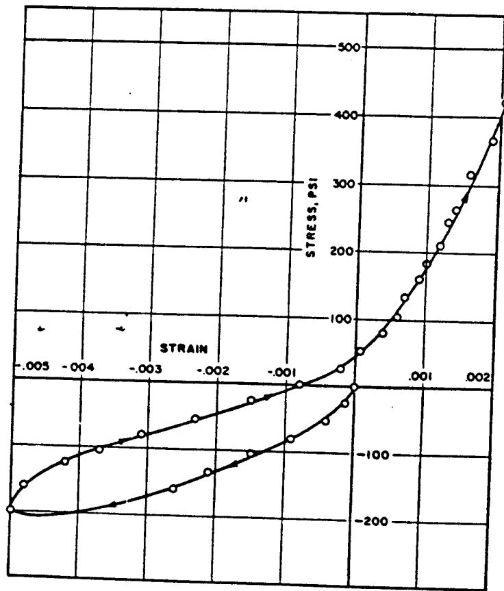
Figure 2.17 Continuous stress-strain curve through compression and into tension for nylon cords embedded in rubber.
