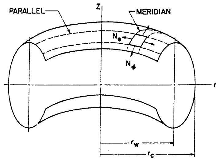
Figure 3.1 Portion of a pressurized toroidal shell.
