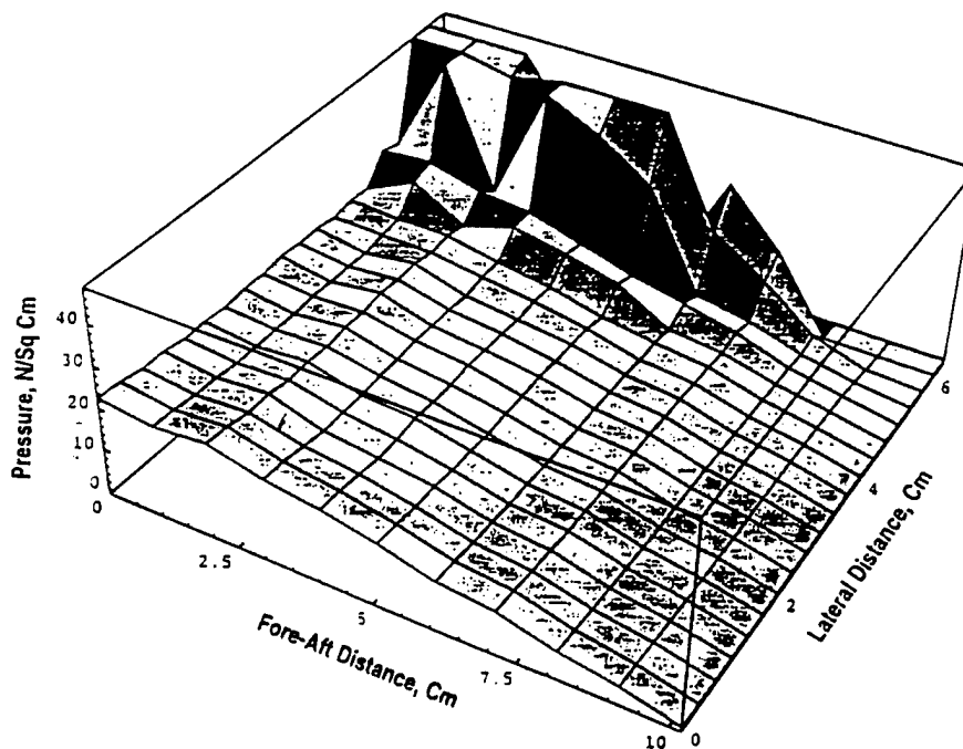
Figure 6.2.12 Ground Pressure Distribution For 34 percent Sidewall Deflection
