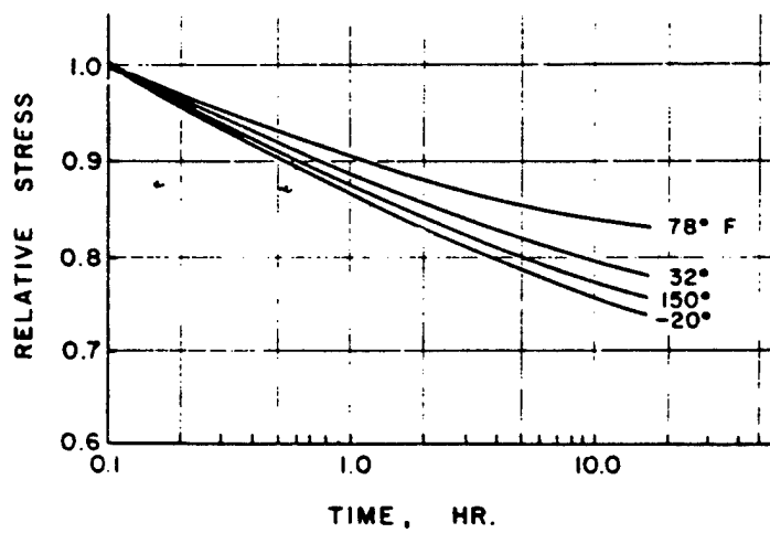
Figure 2.10 Compressive stress relaxation for an SBR tread compound under 30% compression.
