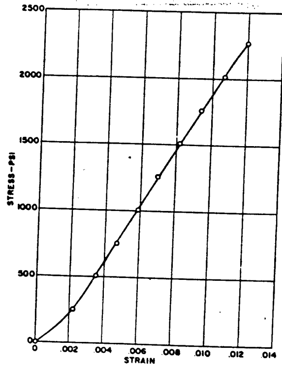
Figure 2.14 Stress-strain curve in tension of rayon cords embedded in rubber, where stress is based on total cross-section area of specimen.
