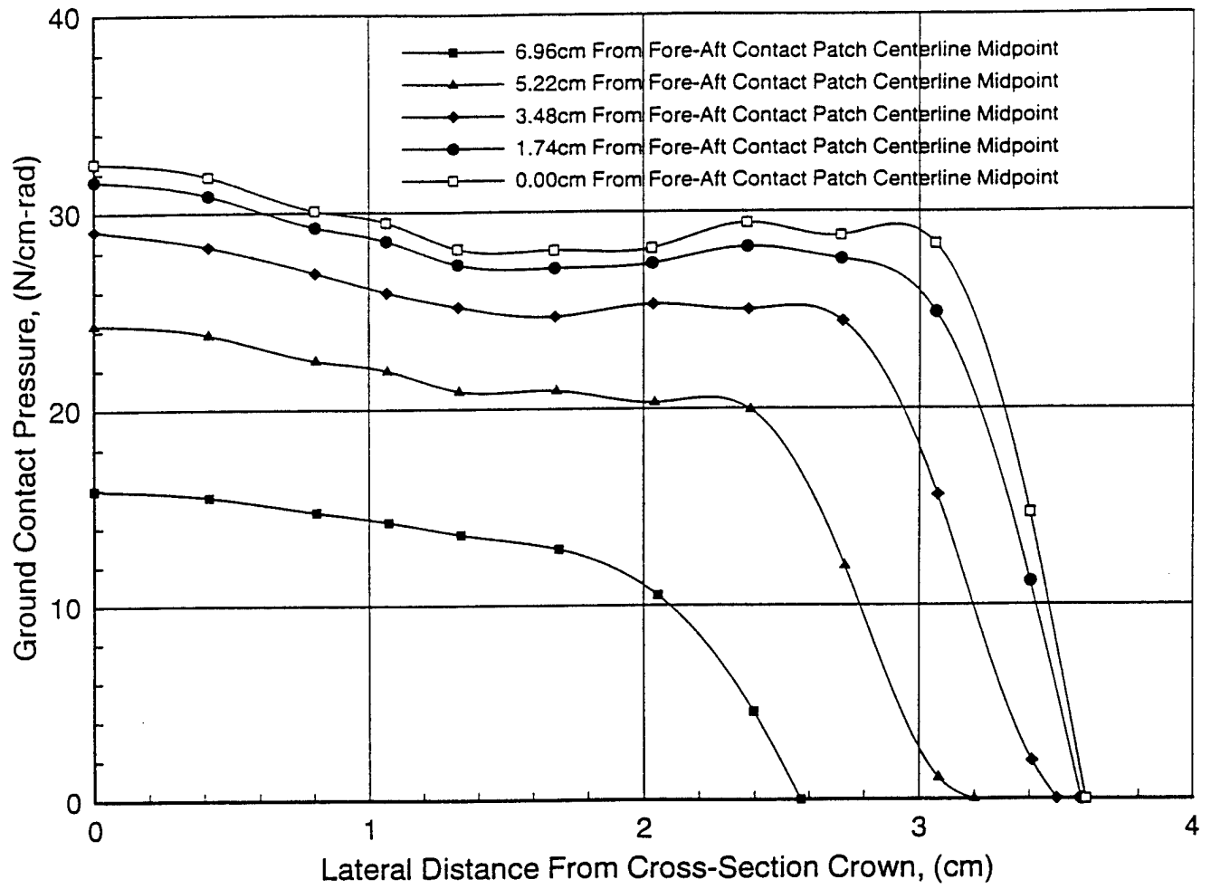
Figure 6.2.14 The Contact Pressure Distribution Variation With Fore-Aft Distance cm From Midpoint of Contact Patch Centerline for 20 percent sidewall deflections
