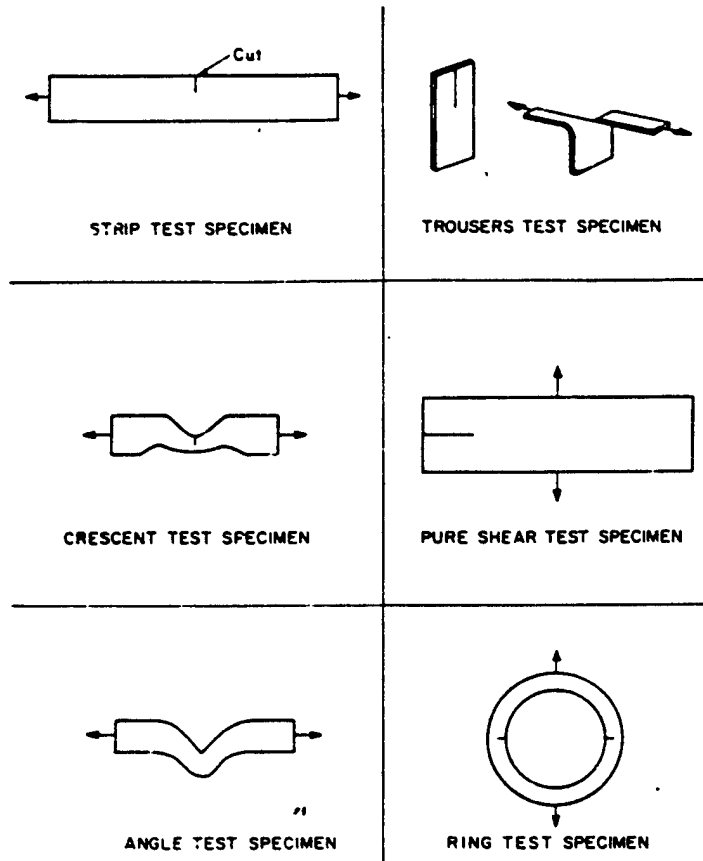
Figure 2.5 Tear test specimens.
