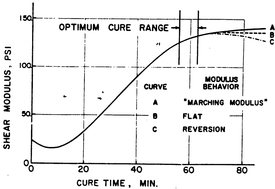
Figure 2.3 Diagram of continuous cure curves.
