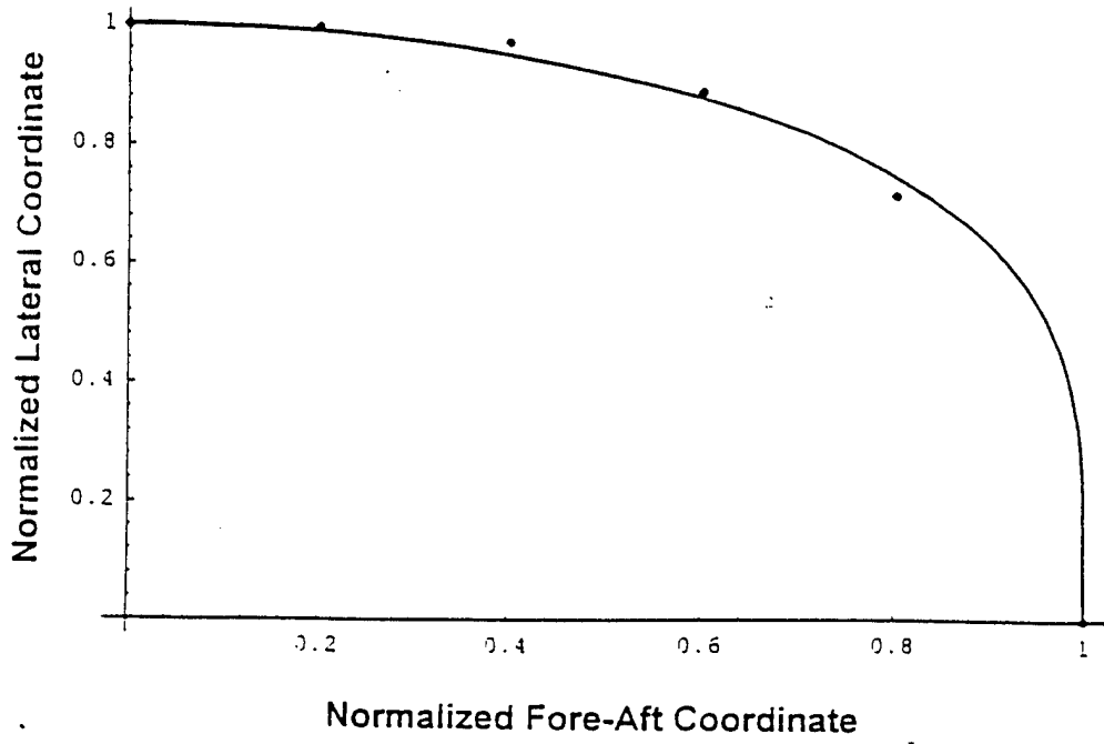
Figure 6.2.9 Foot Print Shape For 20 percent Sidewall Deflection
