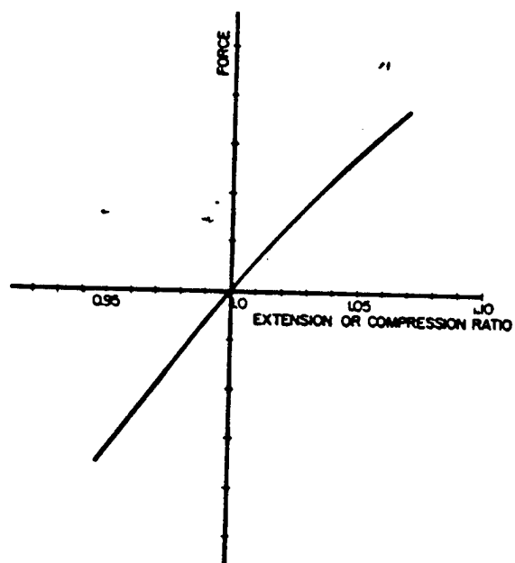
Figure 2.12 Region near origin of force-extension ratio curve for rubber.
