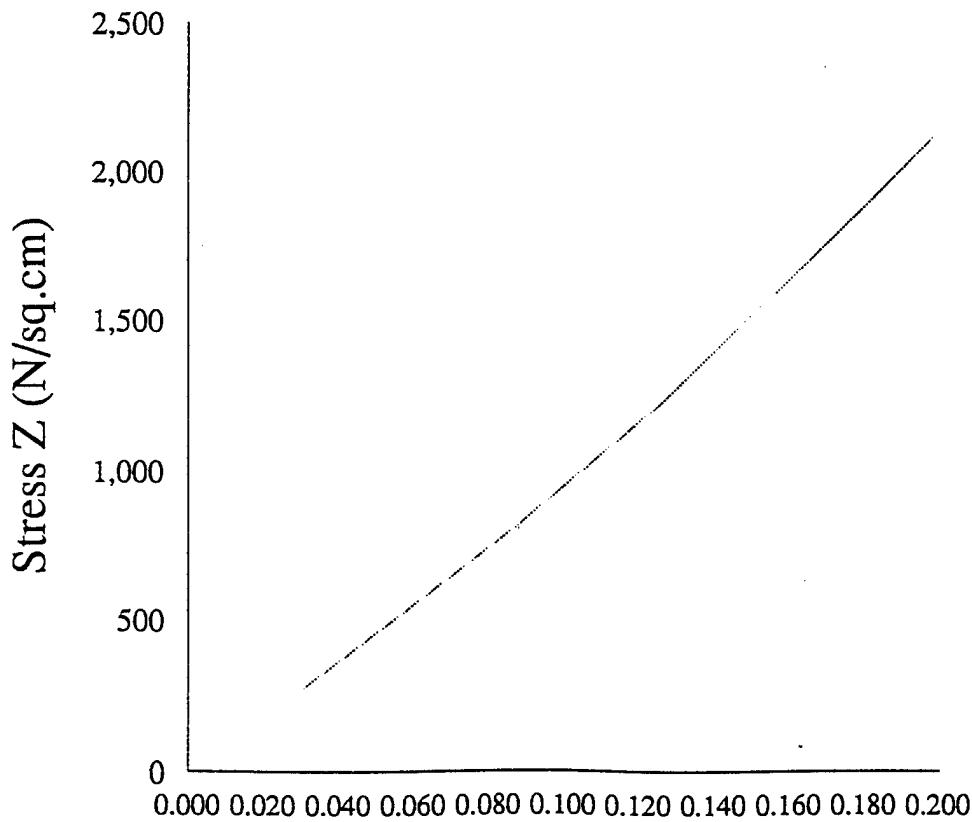
Figure 6.1.6 Stress vs Strain - Thickness Direction - CAX4IH Elements
