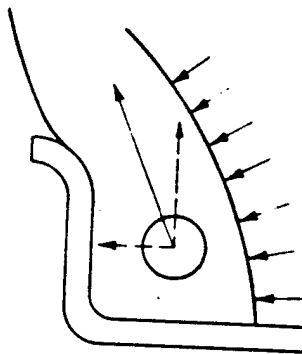
Figure 2.20 Forces pressing bead against rim flange on the wheel to obtain driving and braking reactions.
