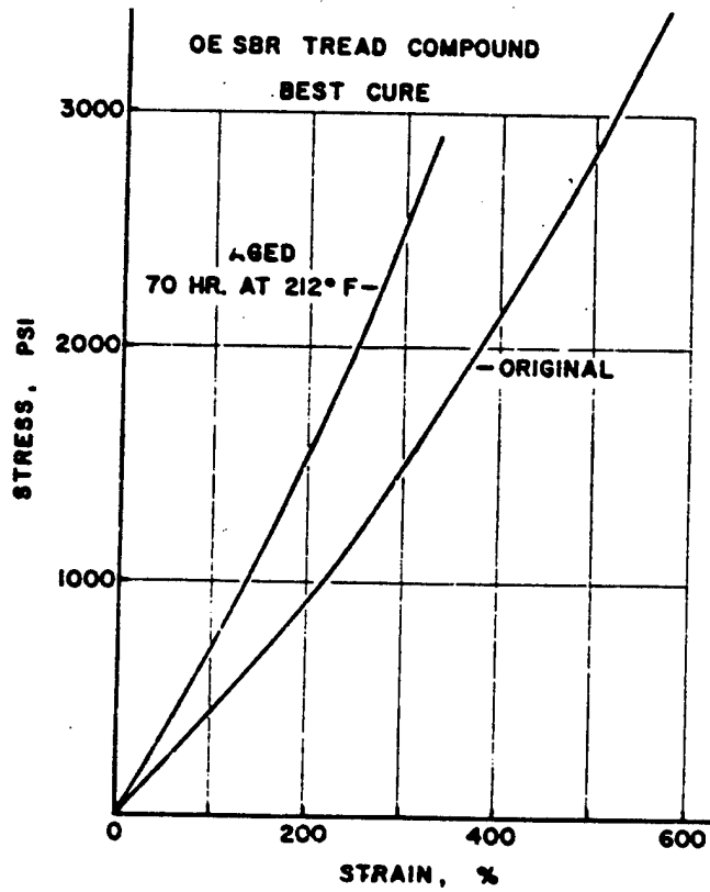
Figure 2.4 Effect of air-oven aging on stress-strain curve of the rubber compound of
