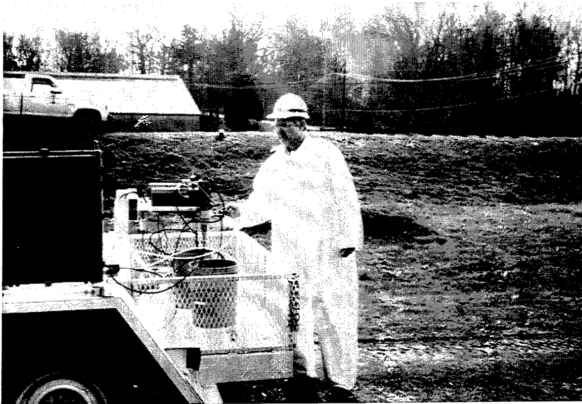
Figure 3. Original SCAPS grouting system utilizing twin airless piston pumps and 1/4-in.-diameter grouting tubes
