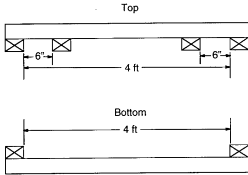
Figure 8. Jigs made from 2- × 4-in. lumber to hold the insulation during installation.
