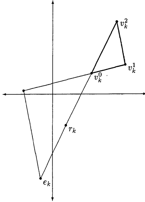
FIG. 3. An expansion step of the straightforward rank ordered pattern search method, given the simplex with vertices \{v_k^0, v_k^1, v_k^2\} .
