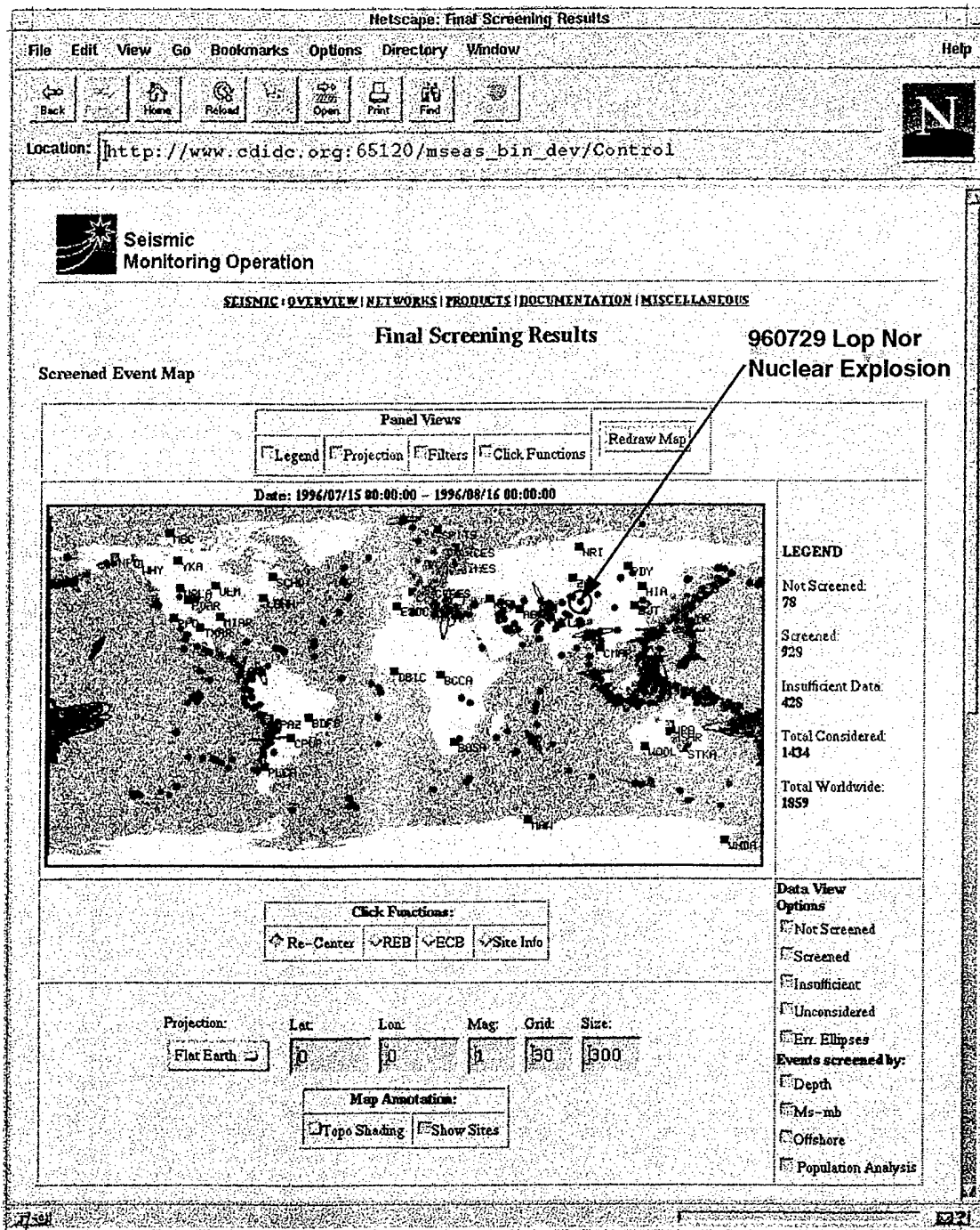
Figure 7. Map showing seismic events, with location error ellipses, and color-coded by their screening results.
