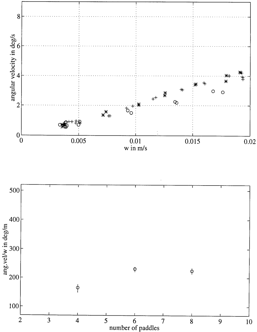
Figure 9: Float rotation rate dependence on the number of vanes — four, six, and eight paddles of 6" sides on 12" arms oriented at 30° to the horizontal. The top panel shows \omega against w for the three cases. The bottom panel shows the mean slope for each of the three curves of \omega vs. w in the top panel. This slope is the "sensitivity", \omega/w , of the float for a given set of parameters. The error bars in the bottom panel represent the 95% confidence interval of the slope.
