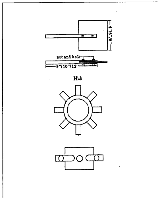
Figure 2: Plan and side view of the vane assembly. The vane is made up of a square plastic paddle screwed onto a PVC arm. The vanes are then press-fitted into the hub, which is taped onto the body of the float (see Figure 1).
