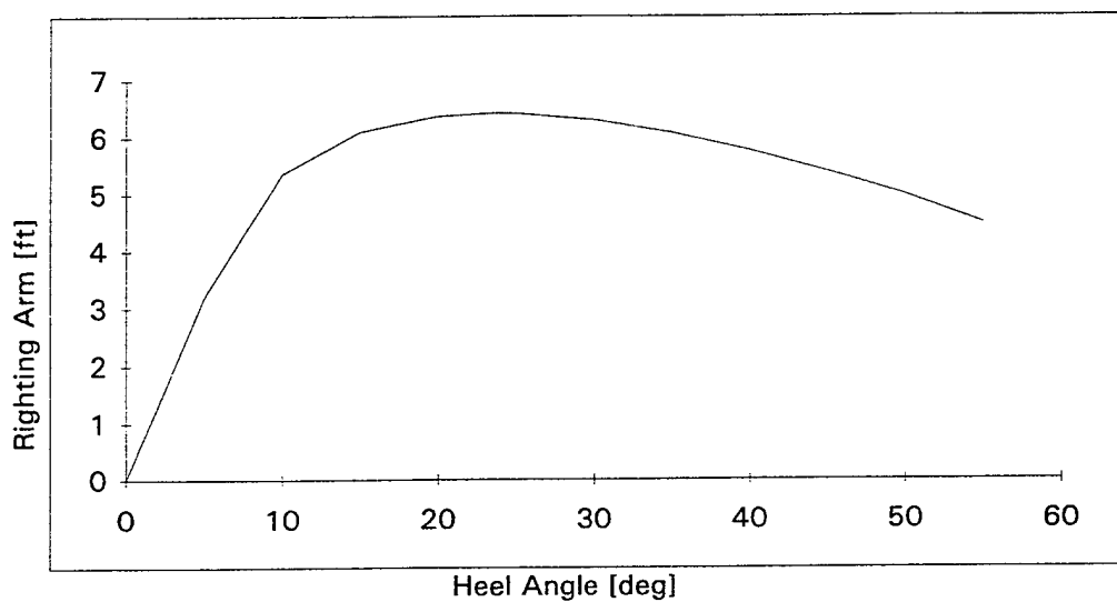
FIGURE 4.12 RIGHTING ARM CURVE FOR UNLOADED 120 FT BARGE
