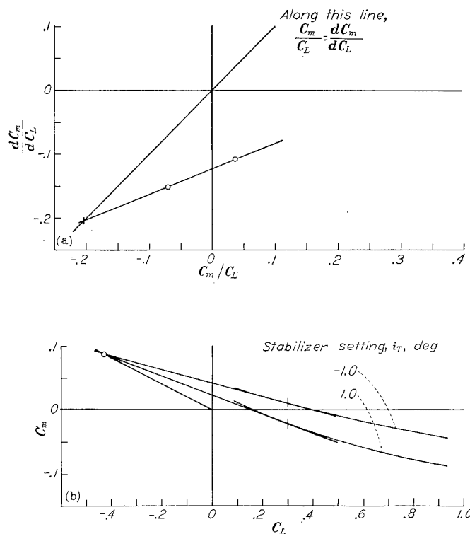
(a) Method of extrapolation of slopes. (b) Method of tangents. FIGURE 50.—Graphical procedures for determination of stick-fixed neutral point from wind-tunnel tests.
