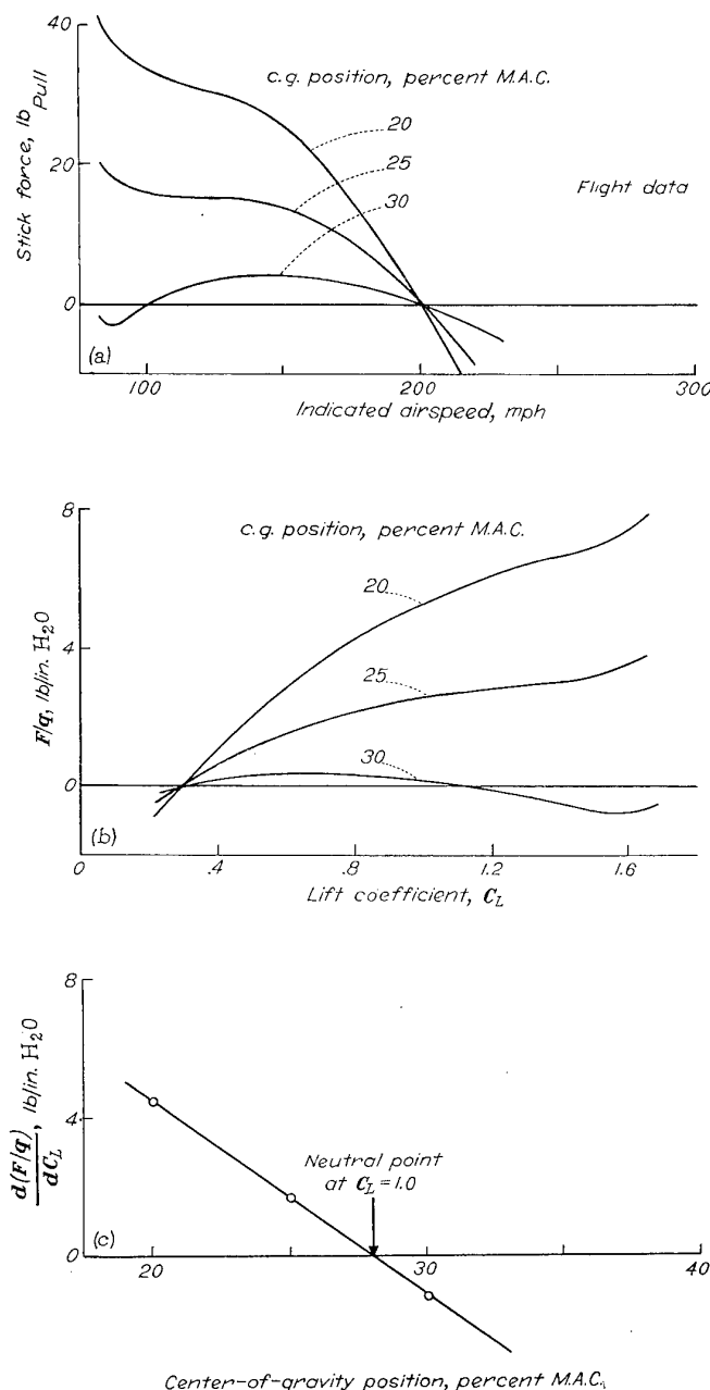
(a) Variation of stick force with indicated airspeed. (b) Variation of the quantity F/q with lift coefficient. (c) Variation of the quantity \frac{d(F/q)}{dC_L} with center-of-gravity position.
