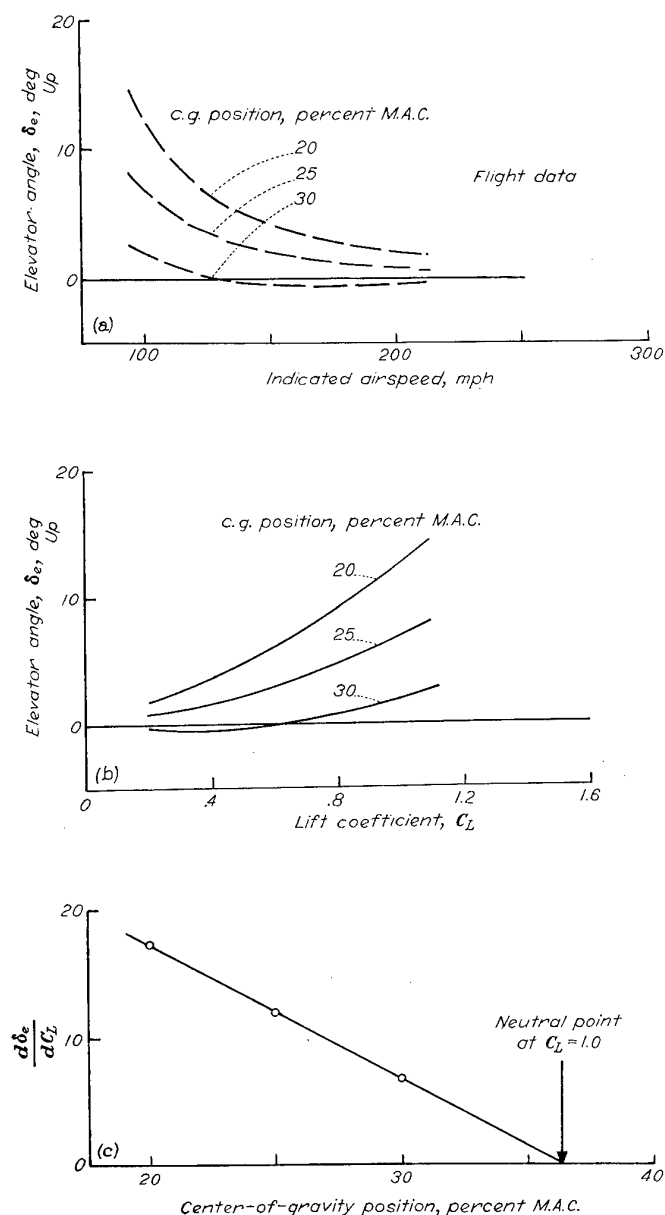
(a) Variation of elevator angle with indicated airspeed. (b) Variation of elevator angle with lift coefficient. (c) Variation of the quantity \frac{d\delta_e}{dC_L} with center-of-gravity position.
