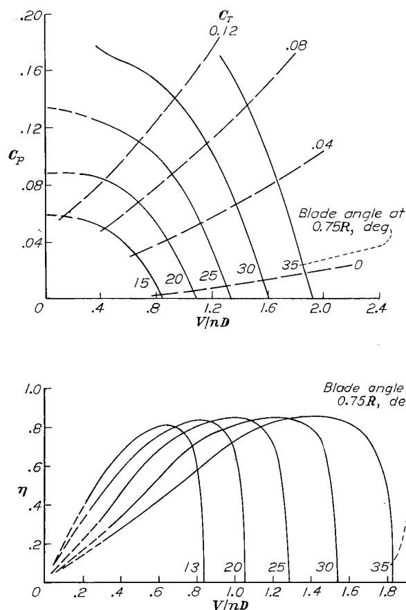
FIGURE 44.—Typical charts showing propeller characteristics.
