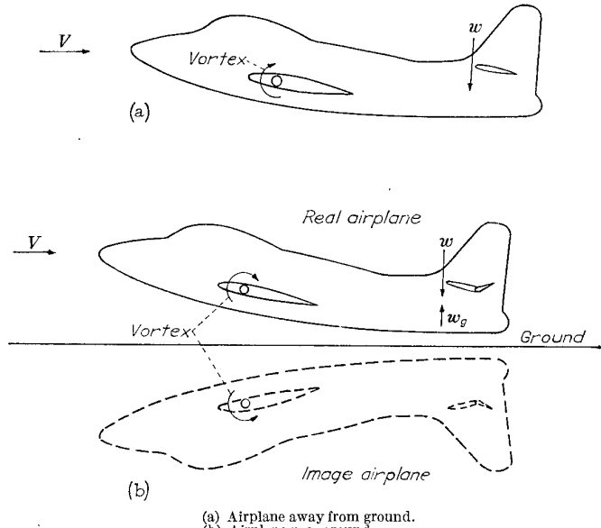
FIGURE 15.—Effect of image vortex system on downwash at tail as airplane approaches the ground.
