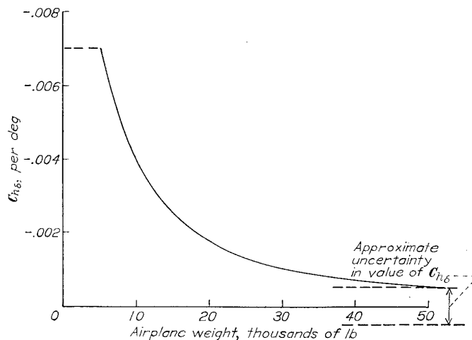
FIGURE 19.—Approximate reduction in C_{h\delta} required to meet elevator-control-force requirements as a function of airplane weight.
