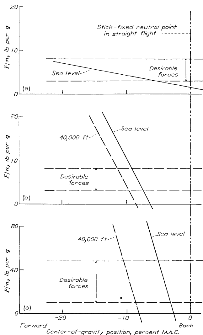
(a) Light airplane. (b) Fighter airplane. (c) Bomber. FIGURE 18.—Stick-force characteristics in maneuvers for three types of airplanes with unbalanced elevators; airplane characteristics given in table I. C_{h\alpha} = -0.003 per degree C_{h\delta} = -0.007 per degree.
