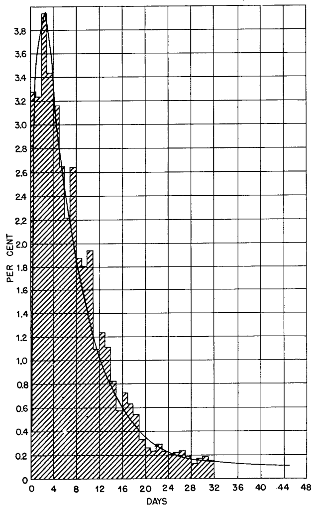
Figure 3. Fecal excretion of Pu by the rat, 15.2 r Pu administered intravenously as PuCl 3 — per cent of dose excreted per day.
