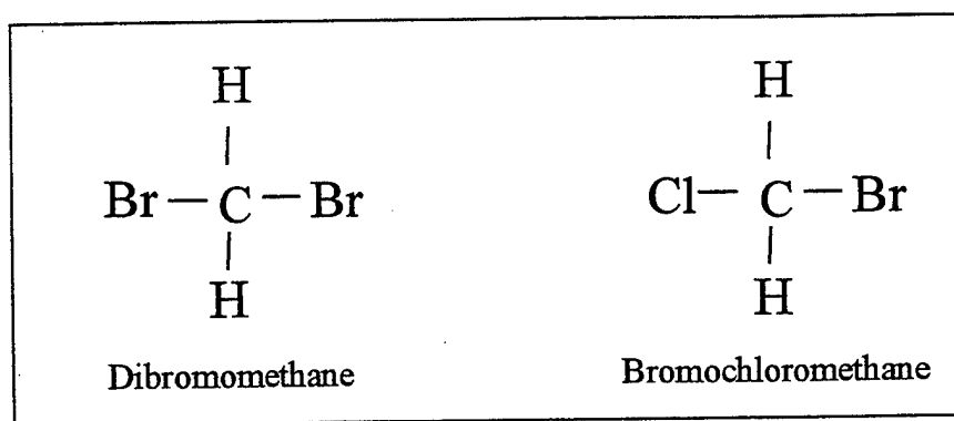
Figure 2. Chemical Structures of Test Chemicals
