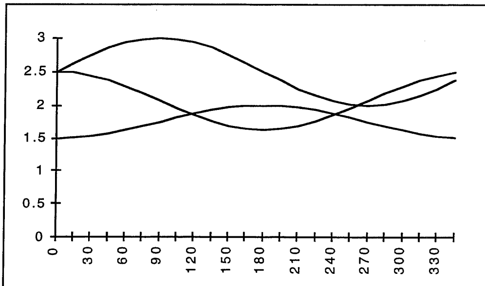
Figure A.10 -- Simulated Magnetometer Data for Elevation = -60°, Roll = 0°
