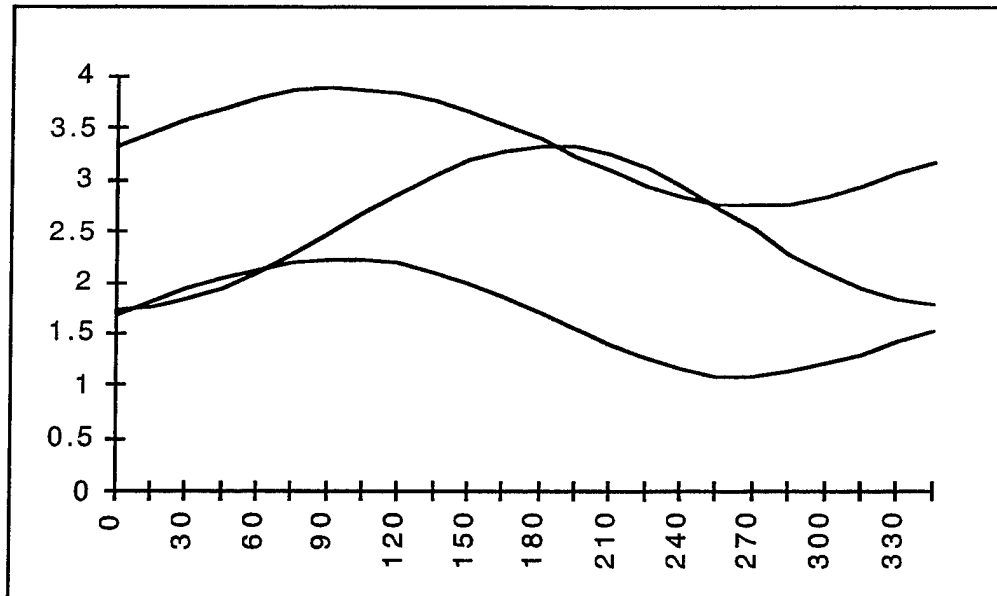
Figure A.17 -- Real Magnetometer Data for Elevation = 0^\circ , Roll = +45^\circ
