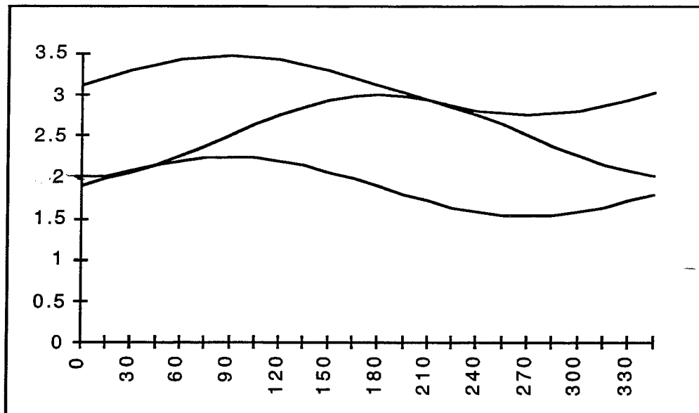
Figure A.18 -- Simulated Magnetometer Data for Elevation = 0^\circ , Roll = +45^\circ
