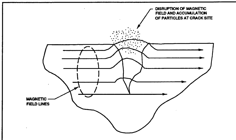
Figure 6. Magnetic particle indication at a surface discontinuity (after AWS (1986))
