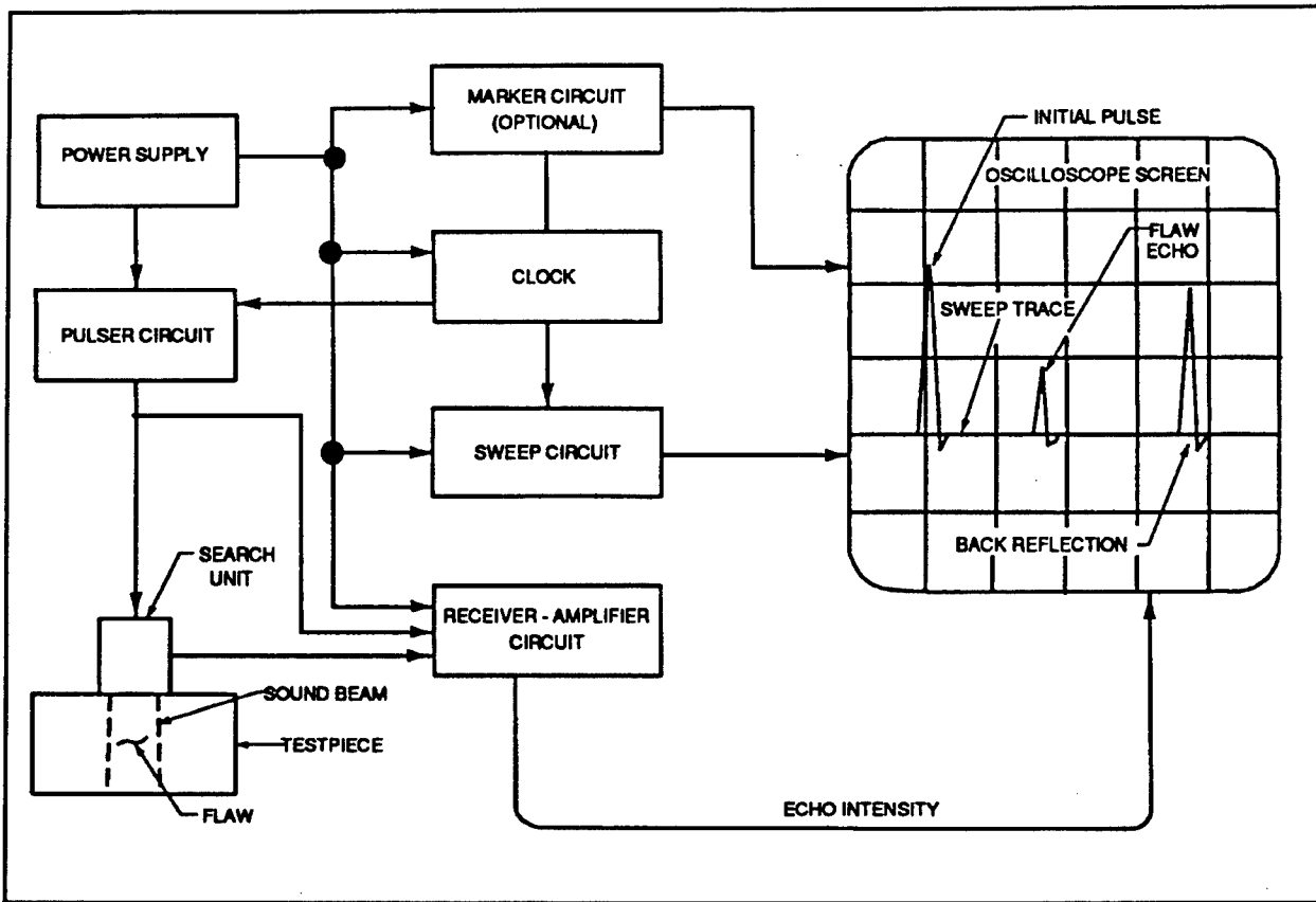
Figure 10. Block diagram of a pulse echo ultrasonic inspection system (after ASM (1989))
