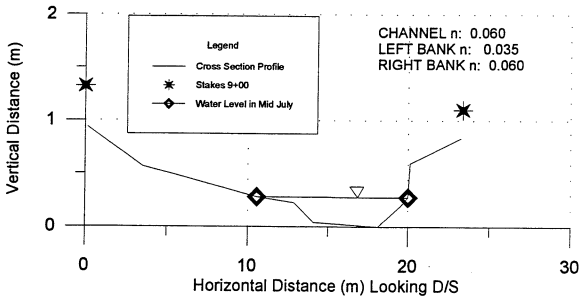
Degraded Reach Cross Section D10
