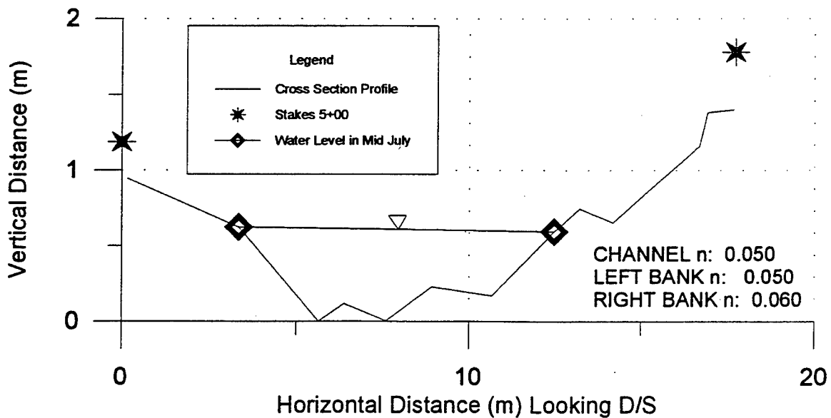
Natural Reach Cross Section N6
