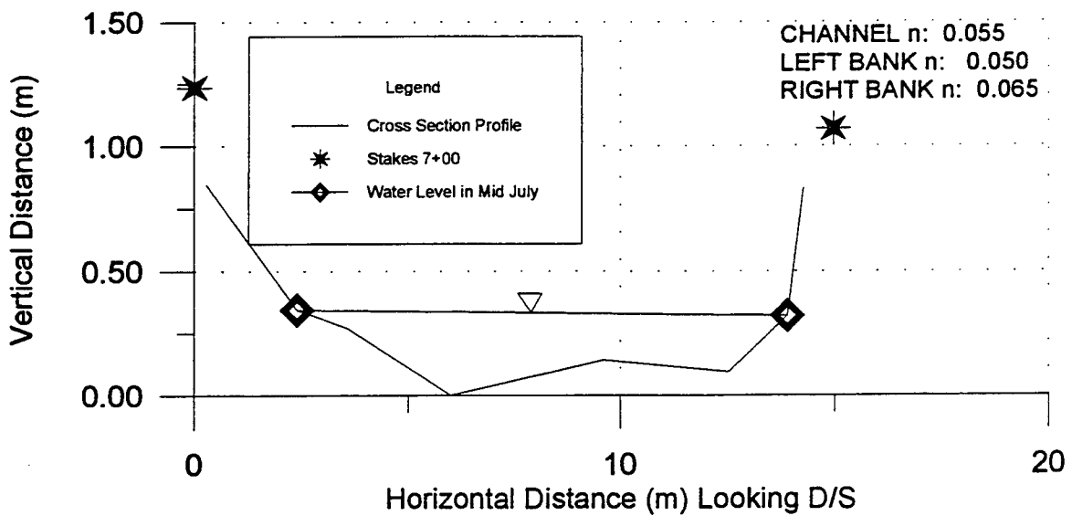
Degraded Reach Cross Section D8
