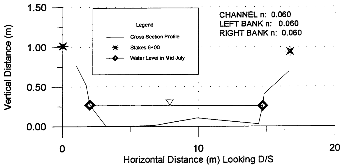
Degraded Reach Cross Section D7
