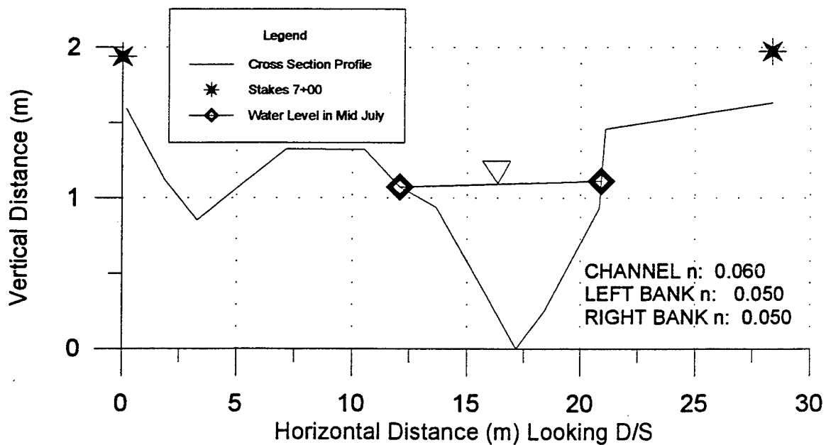
Restored Reach Cross Section R8
