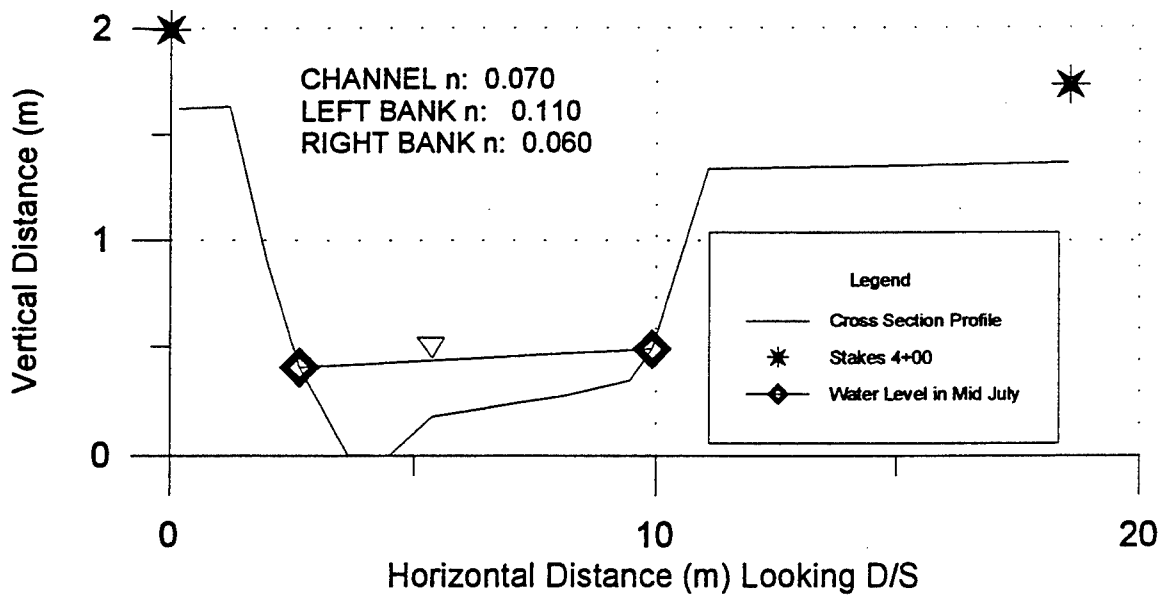
Natural Reach Cross Section N5
