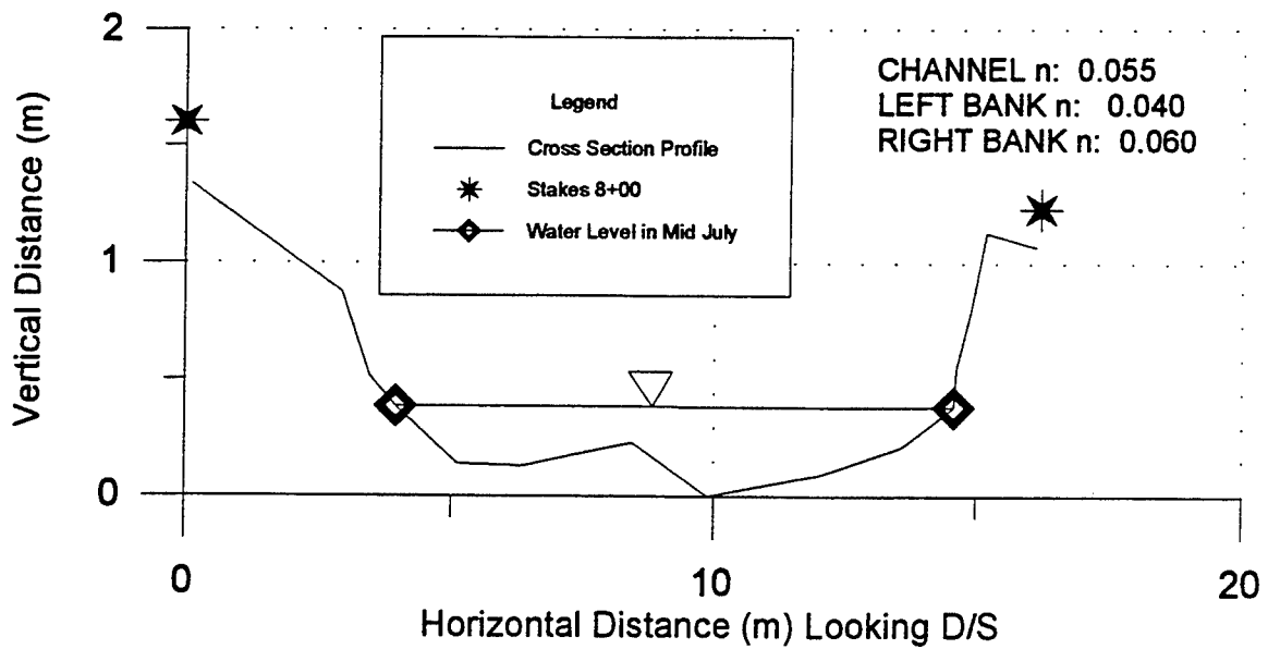
Degraded Reach Cross Section D9
