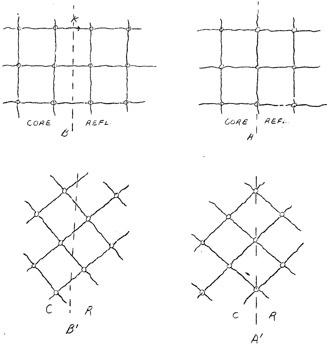
Figure 3. Core-Reflector Boundaries-Schematic
