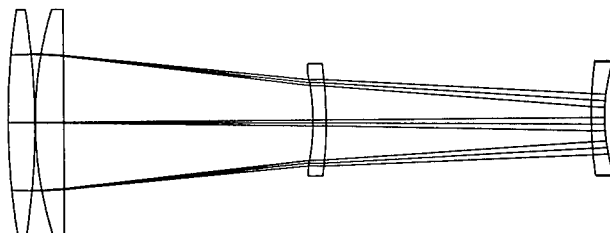
Figure 25. Magnifier optics.
