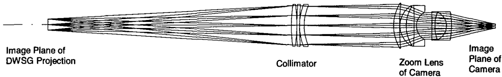
Figure 19. Collimator lens system for DWSG projection.
