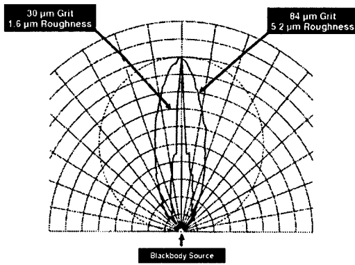
Figure 16. ZnSe samples, blackbody source.
