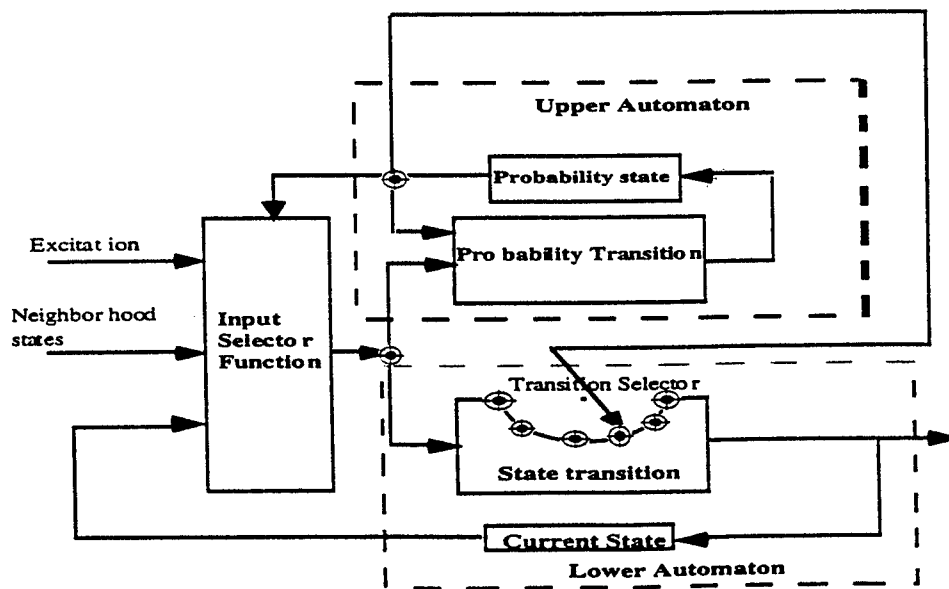
Figure 5. Quantum Particle
