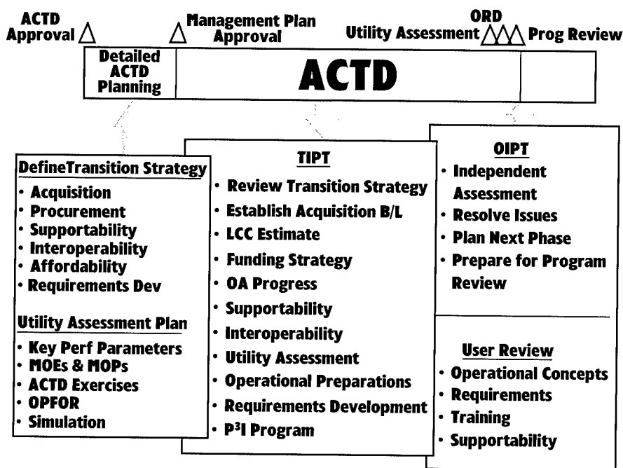
Figure 3. Transition Framework
