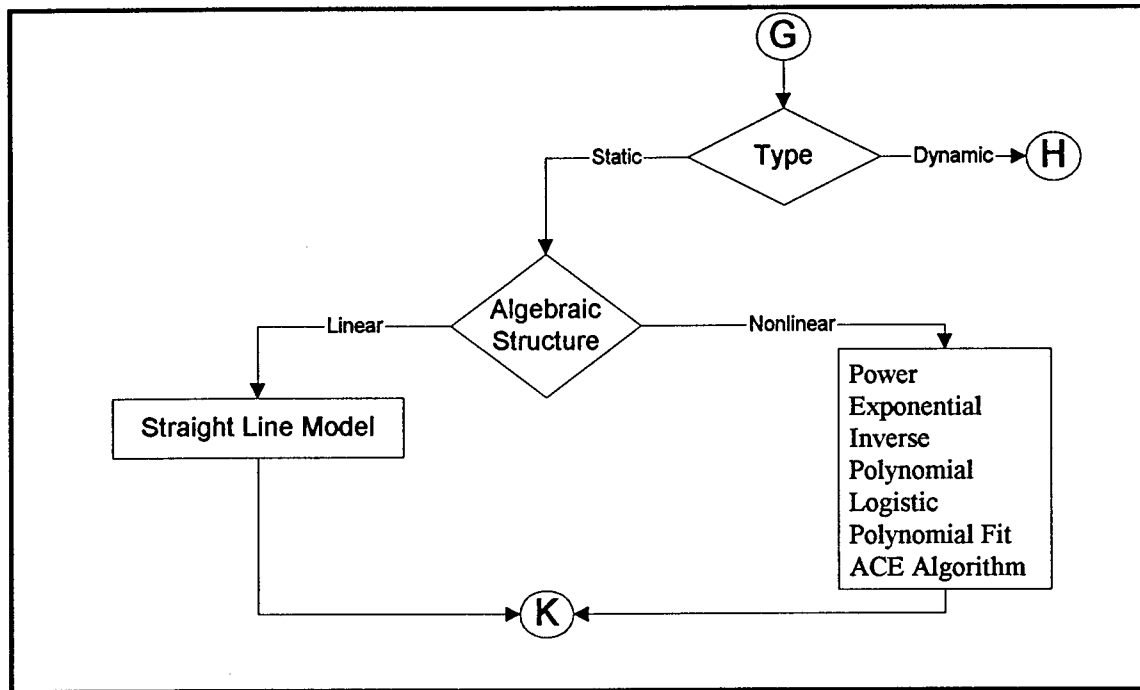
Figure 10.4.8 Metamodel Structure for Static Systems.
