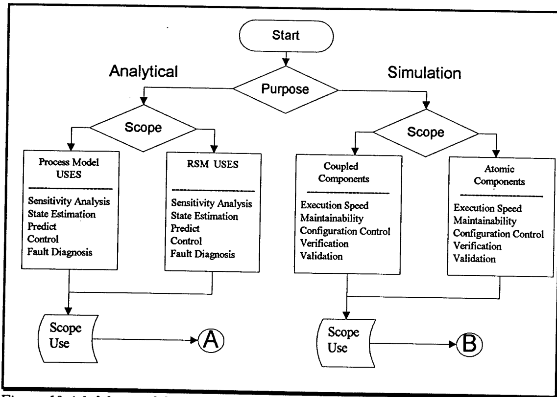
Figure 10.4.1 Metamodeling Approach
