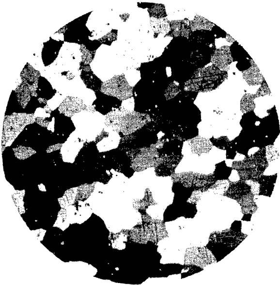
71227 AVERAGE GRAIN DIAMETER 0.062 mm
