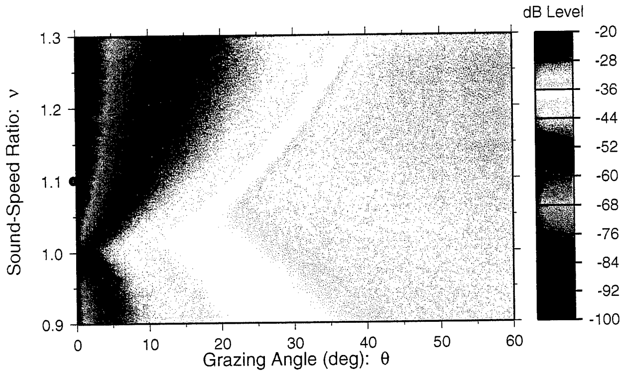
Fig. 5 – Sediment backscatter strength as function of sound-speed ratio \nu and grazing angle \theta . Frequency f = 400 Hz. Environmental parameters: g = 1.0 \text{ s}^{-1} , \rho = 1.5 , \delta = 0.01 , and w_2 = 0.001 \text{ m}^4 . Mark on vertical axis indicates value common to Figs. 2-6.
