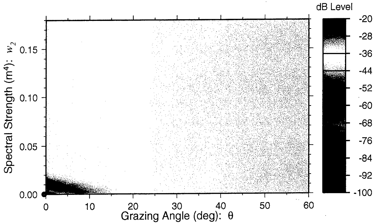
Fig. 3 – Sediment backscatter strength as function of spectral strength w_2 and grazing angle \theta . Frequency f = 400 Hz. Environmental parameters: g = 1.0 \text{ s}^{-1} , \nu = 1.1 , \rho = 1.5 , and \delta = 0.01 . Mark on vertical axis indicates value common to Figs. 2-6.
