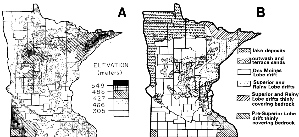
Figure 4. Elevation and soils in Minnesota. The topographic elevation map of Minnesota (A) is drawn from Baker and Strub (1963) and the surficial geological map (B) is adapted from Hogberg (1972). The lake deposits and till from the Des Moines Lobe are primarily calcareous; whereas the deposits and till from the Superior and Rainy Lobe range from noncalcareous to weakly calcareous.
