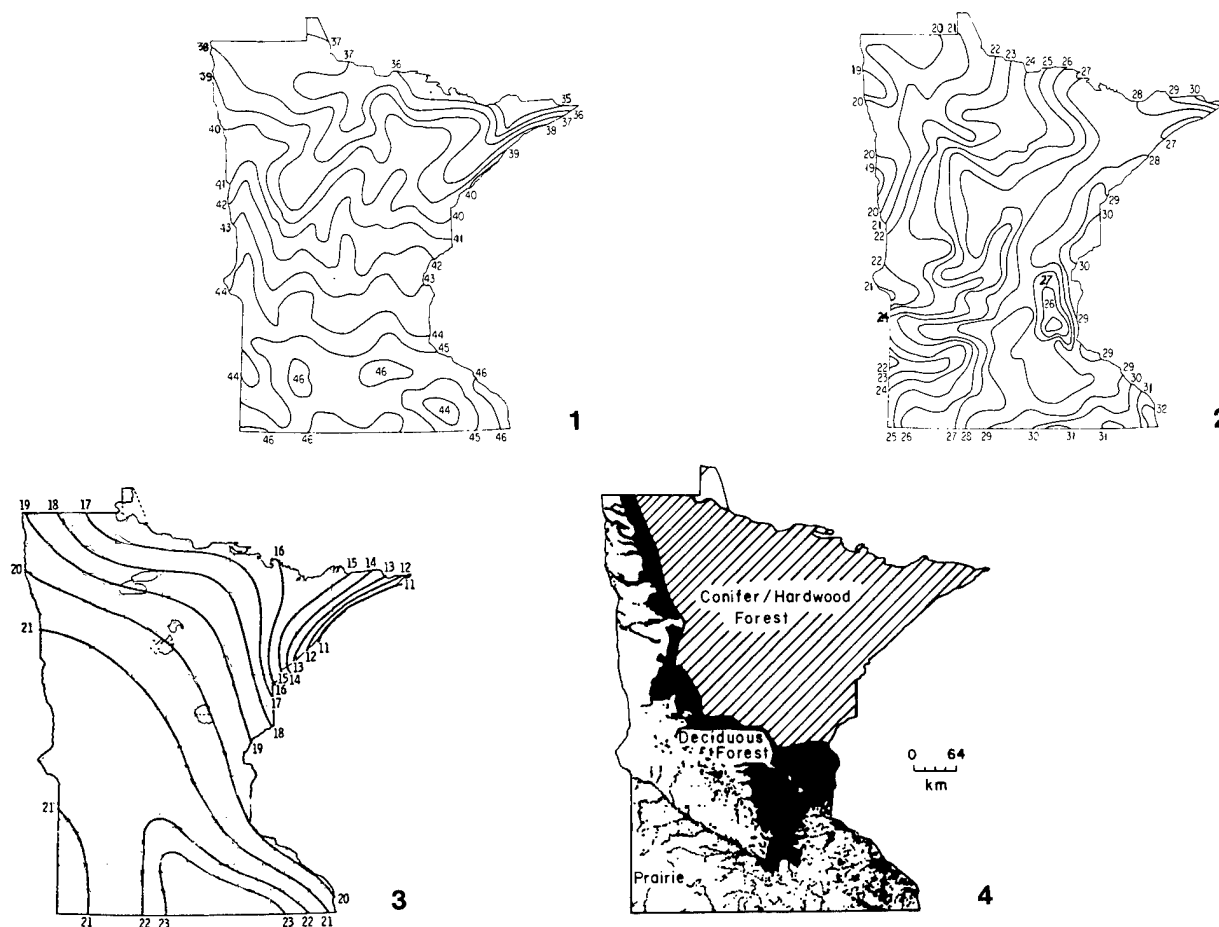
Figure 5. The climate and vegetation of Minnesota: (1) average annual temperature in °F (Baker and Strub 1965), (2) average annual precipitation in inches (Baker et al. 1967), (3) average annual evapotranspiration in inches (Baker et al. 1979), (4) presettlement vegetation of Minnesota (after Marschner map, Heinselman 1974).
