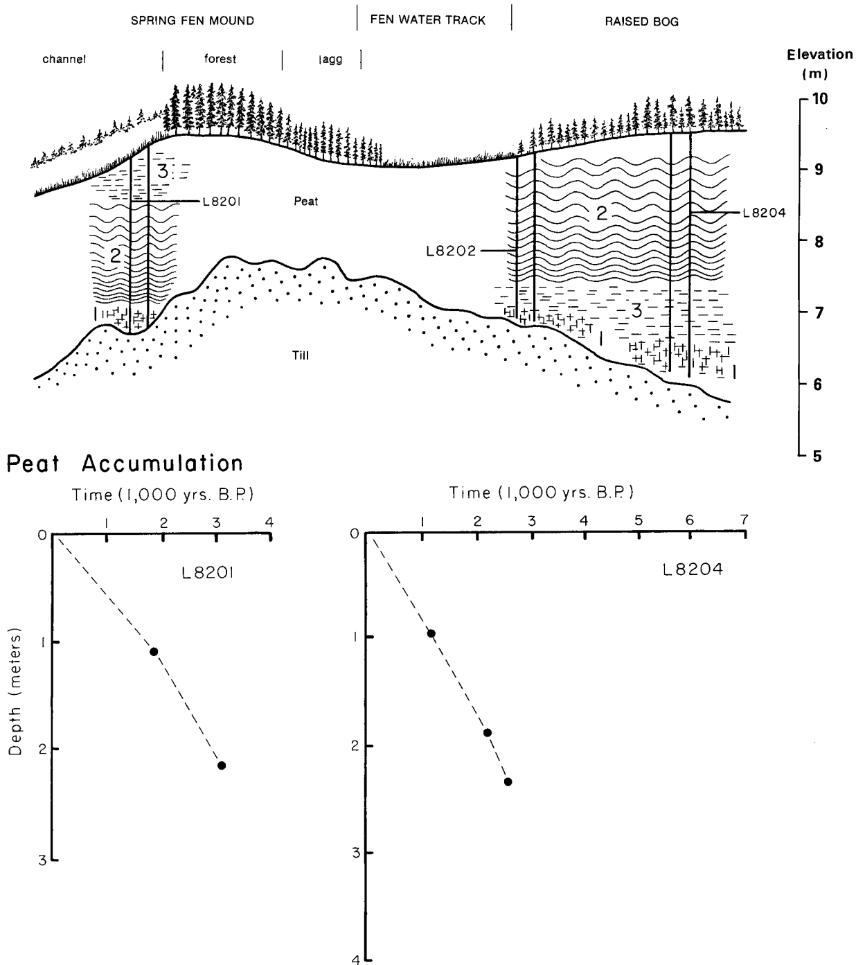
Figure 9. Paludification of sloping ground in the Lost River peatland, northwestern Minnesota. The spring-fen mound has developed over a rise in the mineral substrate, whereas the raised bog has grown over a depression (Almendinger et al. 1986). The peat stratigraphy from the three cores (L8201, L8204, and L8202) indicates that deeply decomposed fen peats (1) first accumulated in the peatland followed by Sphagnum peat with wood (2). In the upper 70 cm of the spring-fen core, however, woody Sphagnum peat is abruptly replaced by sedge-fen peat (3) indicating an abrupt change in the vegetation (Glaser et al., In prep.). Thus the spring-fen mound was once covered by a Sphagnum -dominated bog or poor fen that was abruptly replaced by a spring-fen channel less than 2,000 years ago. The cores in this diagram were collected adjacent to those in Figures 6, 7, and 8.
