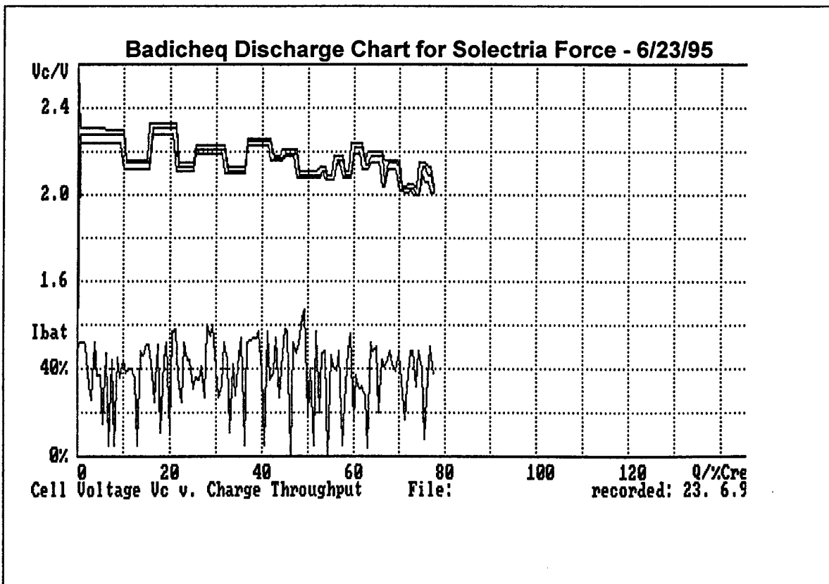
Figure 8 Badicheq discharge chart
