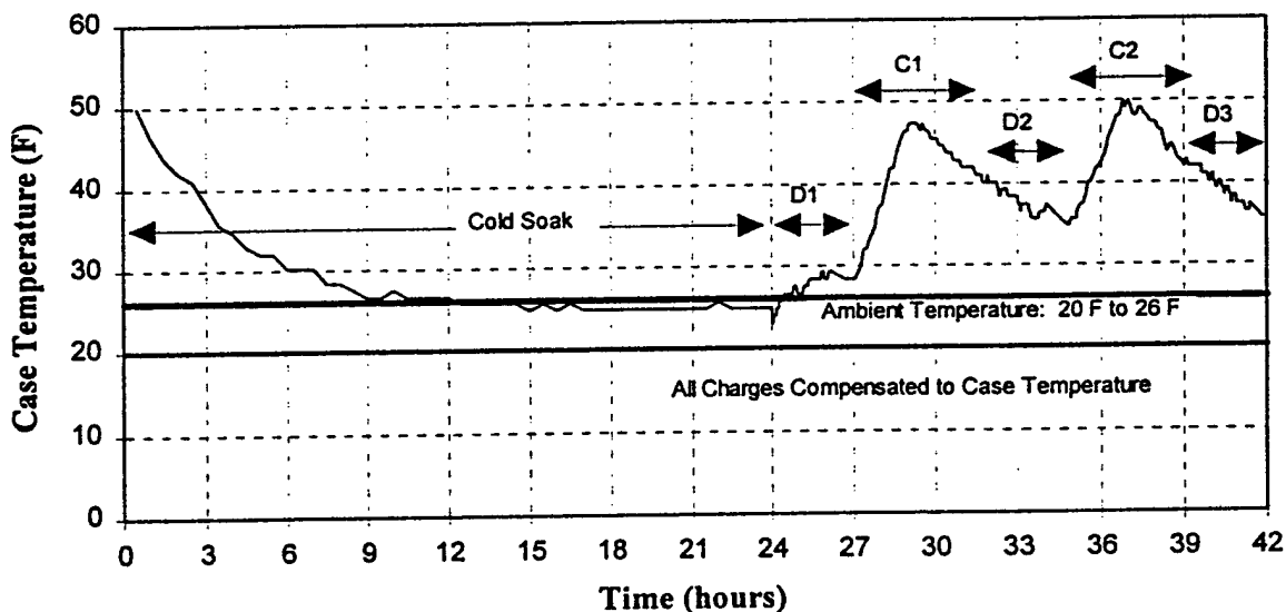
Figure 6 Ambient and Battery Case Temperature
