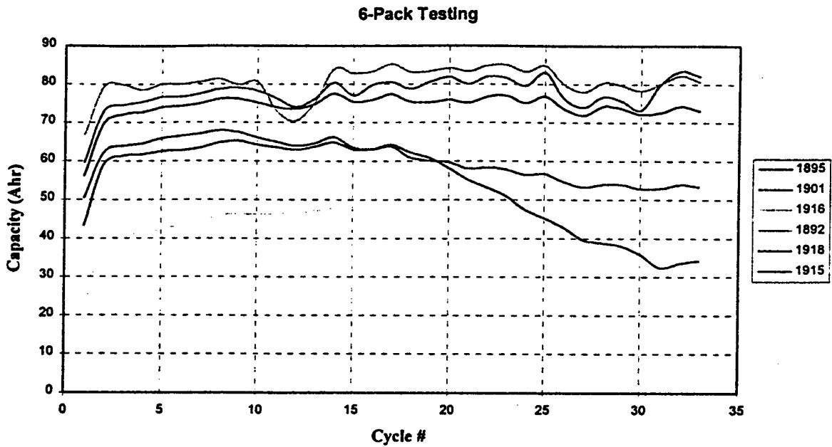
Figure 12 Module Group 2A Amp Hours Versus Cycles
