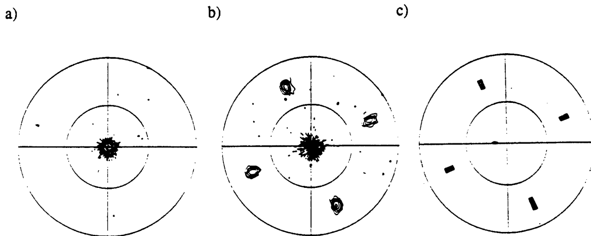
Fig. 3 XRD-polefigures of a) (002)- and b) (110) \text{BaCe}_{0.5}\text{Zr}_{0.5}\text{O}_3 and c) (110) \text{SrTiO}_3 demonstrate the in-plane orientation relationship [100]\text{film} \parallel [100]\text{substrate} between the solid-solution film and the substrate.
