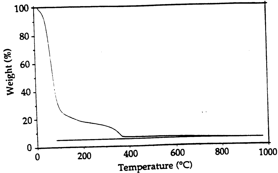
Fig. 1 TGA of a SrZrO 3 -precursor shows the high weight loss during the evaporation of solvent ( T < 100^\circ\text{C} ) and pyrolysis ( T < 400^\circ\text{C} ).
