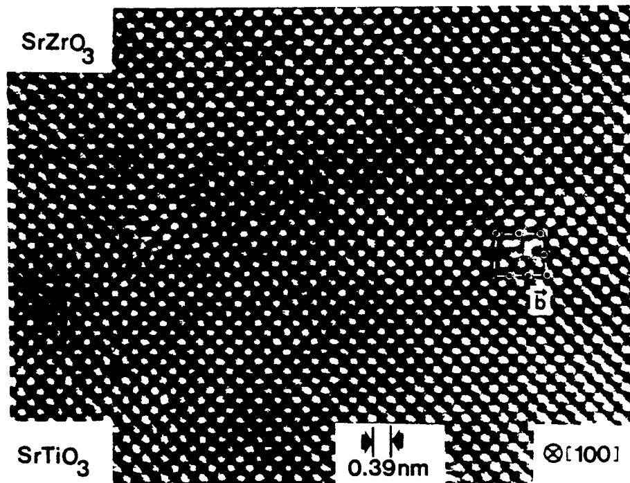
Fig. 5 HREM-image of SrZrO 3 on SrTiO 3 (900°C/1h) in <100> zone-axis shows periodically ordered dislocations.
