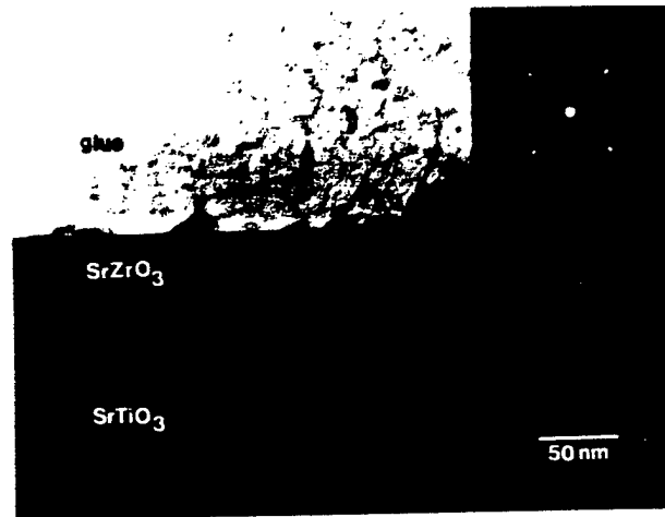
Fig. 4 CTEM-micrograph of a cross-section sample of SrZrO 3 on SrTiO 3 , annealed at 900°C (1h). SAD shows the epitaxial orientation of the film.
