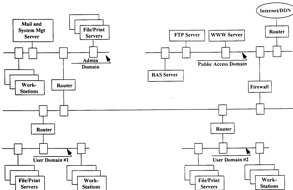
Figure 2.2.1-4 Recommended Architecture
