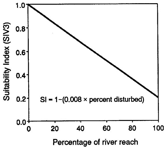
Fig. 2. Suitability index (SIV3)—the relation between the percentage of disturbed river reach and the SI value.
