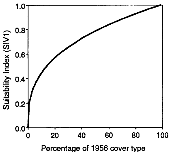
Fig. 1. Suitability index (SIV1)—the relation between the percentage of 1956 cover type and the SI value, determined as: SI = 0.194 \times (\% \text{ of } 1956)^{0.357} . If the observed cover exceeds 100%, the SI should be set at 1.0.
