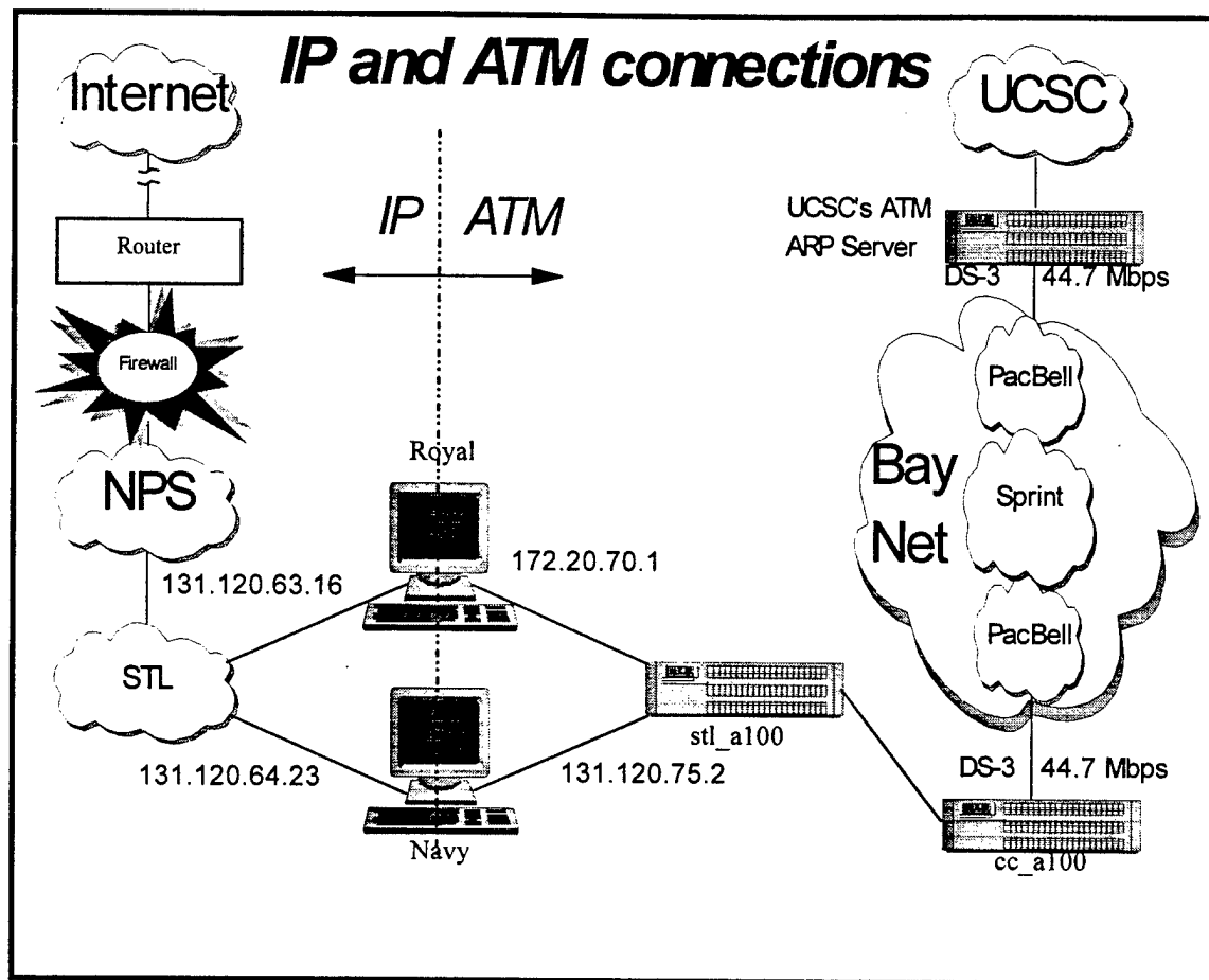
Figure 9. IP/ATM LAN/WAN topology. From (Courtney, 1996).
