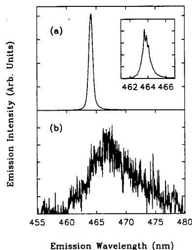
FIG. 2. Typical emission spectra from a \text{ZnS}_{0.05}\text{Se}_{0.95} sample with a cavity length of 399\text{ }\mu\text{m} pumped at 459 nm with pump power densities of (a) 1.4I_{th} and (b) 0.76I_{th} . The threshold pump power density I_{th} was determined to be 350\text{ kW/cm}^2 . The inset shows the longitudinal modes.
