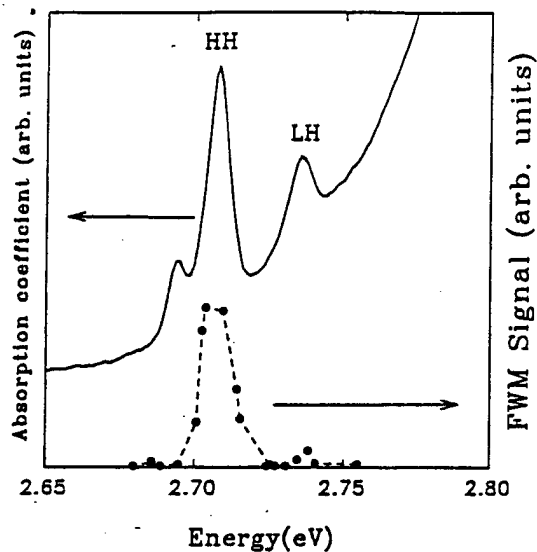
FIG. 2. FWM signal at T=200 fs as a function of the center laser energy for a 6(\text{Zn}_{0.88}\text{Cd}_{0.12}\text{Se}/\text{ZnSe}, 50 \text{ \AA}/250 \text{ \AA}) MQW sample. The top curve shows the absorption spectrum for the MQW.
