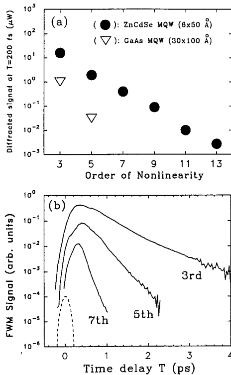
FIG. 1. (a) Average power ( \mu W ) of the diffracted signals at T = 200 fs and 10 K plotted against the order of nonlinearity for a 6 \times (Zn_{0.88}Cd_{0.12}Se/ZnSe, 50 \text{ \AA}/250 \text{ \AA}) MQW grown on ZnSe ( \bullet ), and for a GaAs MQW with 30 \times (GaAs/Al_{0.3}Ga_{0.7}As, 100 \text{ \AA}/100 \text{ \AA}) ( \nabla ). The blue pulse shape (broken lines) is obtained by cross correlating the second harmonic with the primary infrared beam. The 100 fs pulses with an average power of 10 mW per beam are tuned to the HH resonance of the ZnCdSe MQW (2.71 eV) or to that of the GaAs MQW (1.56 eV). (b) Semilogarithmic plot of diffracted signals for the ZnCdSe MQW as a function of T . The experimental conditions are nearly identical to those of (a). The third, fifth, and seventh order signals are shown.
