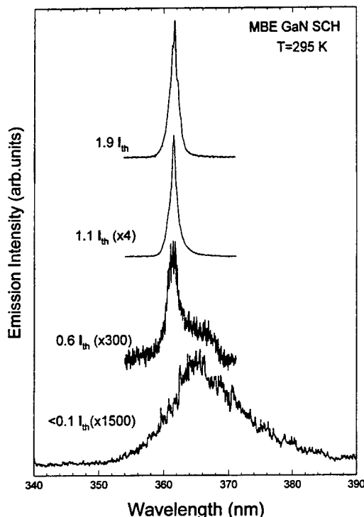
FIG. 1. Emission spectra taken from a GaN/AlGaIn SCH sample at different pumping power densities. The spectra were vertically displaced for the clarification. I_{th} ( =90 \text{ kW/cm}^2 ) represents the pumping threshold for stimulated emission.
