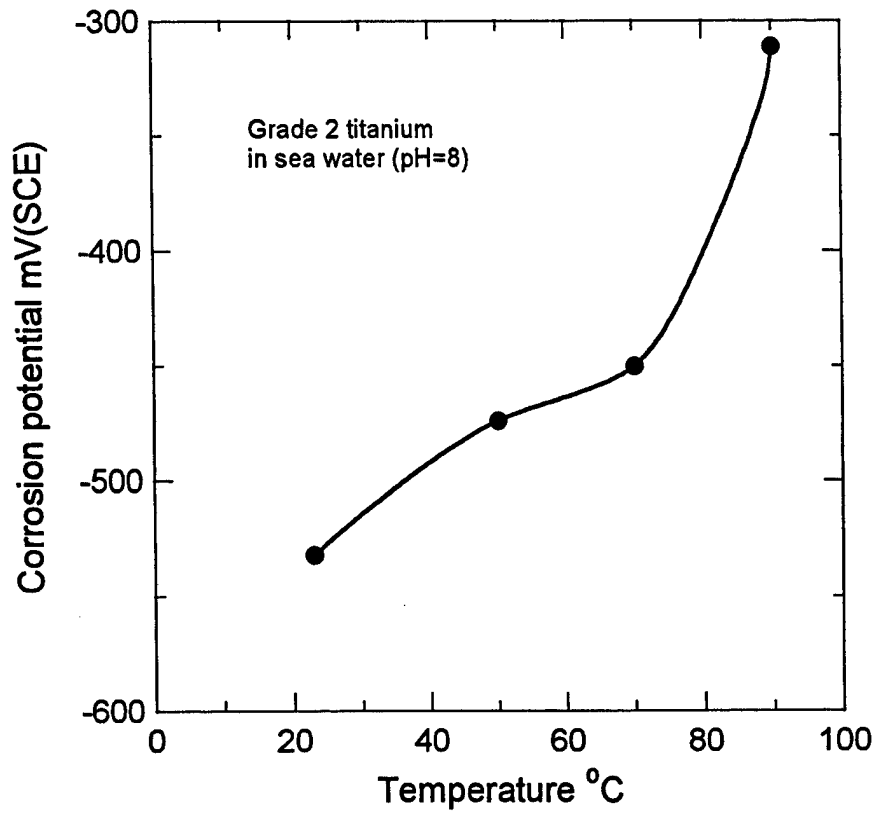
Figure 16 - The variation of the corrosion potential with temperature for titanium in sea water.
