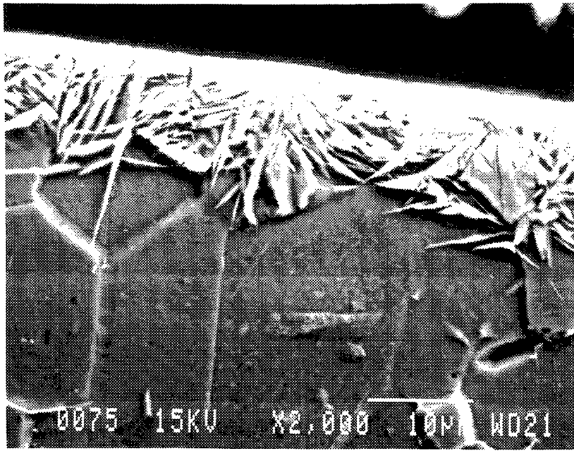
Figure 39 - Microstructure of hydride on the sample surface after the sample was charged in 6%NaCl solution with a current density of 0.5A/cm^2 for 12 hours.
