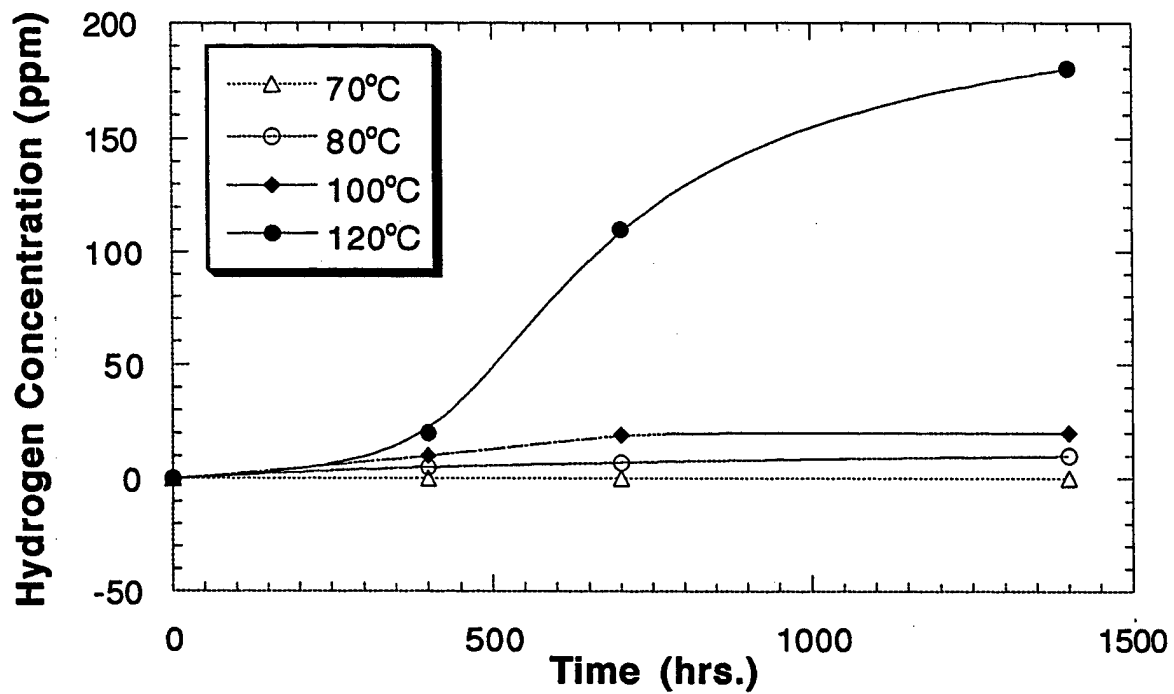
Figure 6 - The hydrogen concentration plotted as a function of time for samples of commercial purity titanium galvanically coupled with steel. Results are given for four different temperatures. The solution was 6%NaCl and the pH was 6. Data taken from reference 8.
