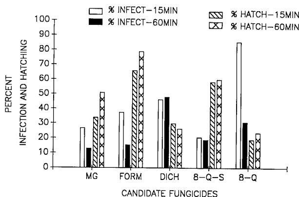
Figure. Relative percent fungal infection of rainbow trout eggs after treatment with candidate fungicides and resulting hatching success. MG = malachite green; FORM = formalin; DICH = dichlorophen; 8-Q-S = 8-quinolinol sulfate; and 8-Q = 8-quinolinol.
