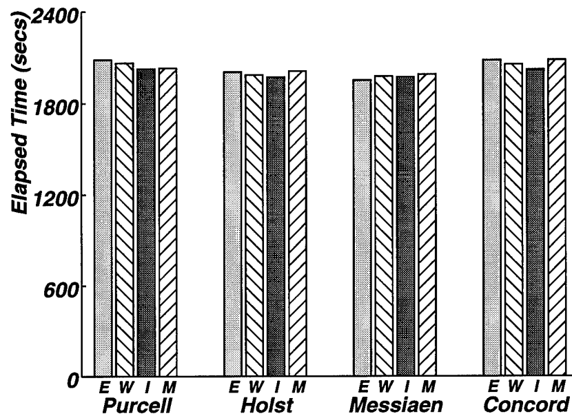
Figure 7.18: Performance of Trace Replay ( \lambda = 1 second, A = 600 seconds)
