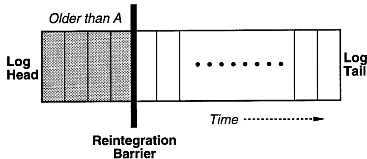
Figure 5.2: CML During Trickle Reintegration
