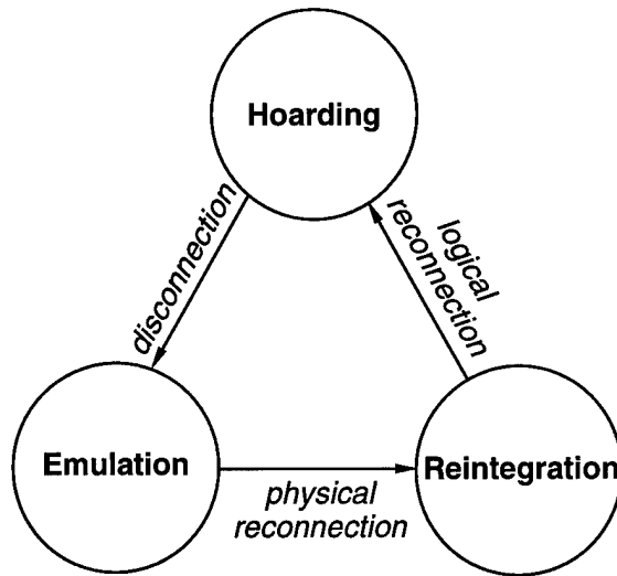
Figure 2.1: Venus State Transition Diagram
