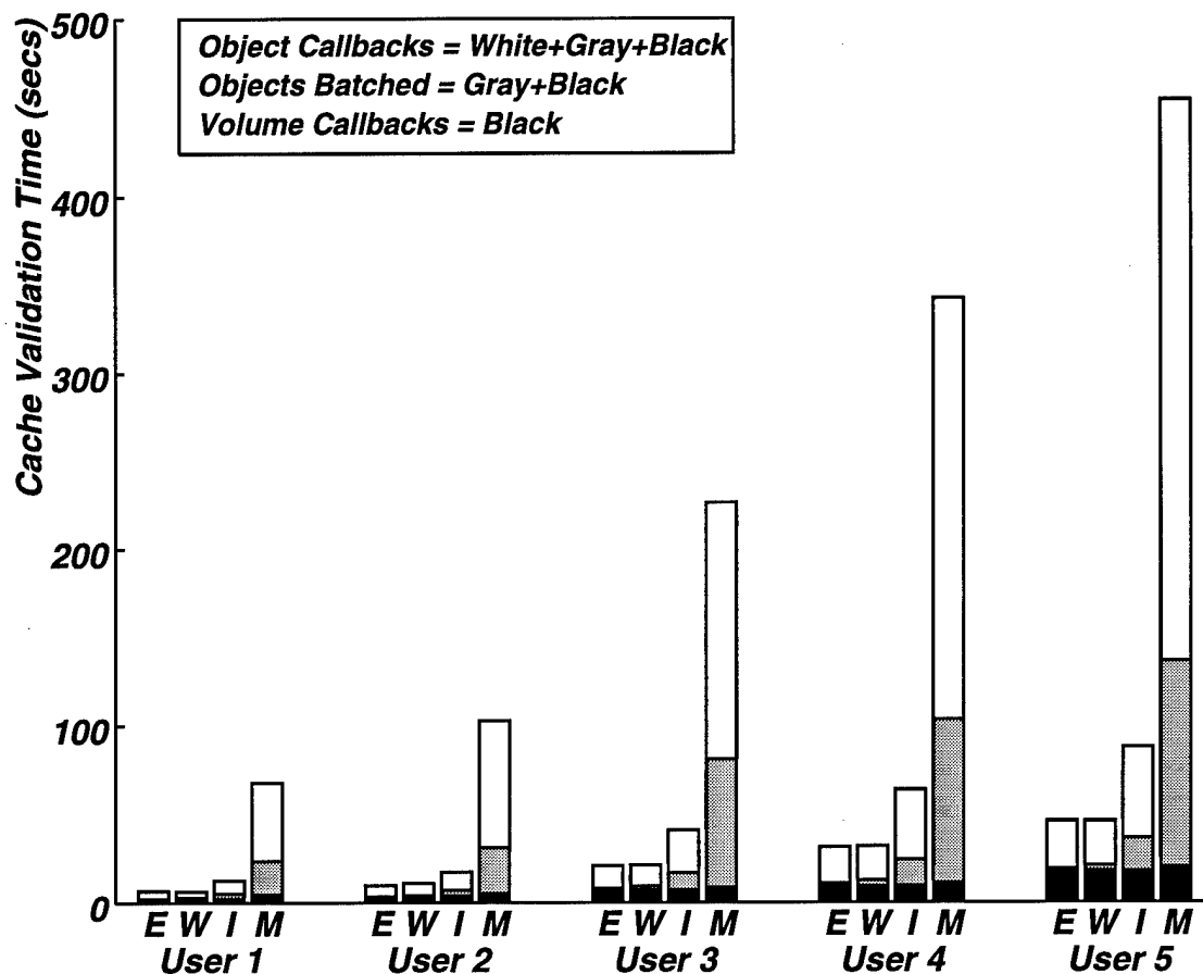
Figure 7.6: Validation Time Under Ideal Conditions
