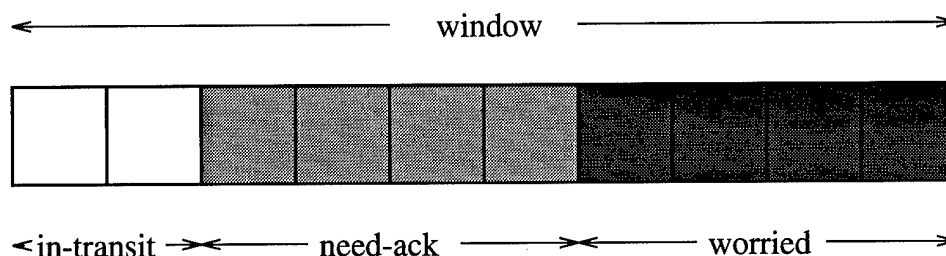
Figure 3.7: SFTP Packet Sets
