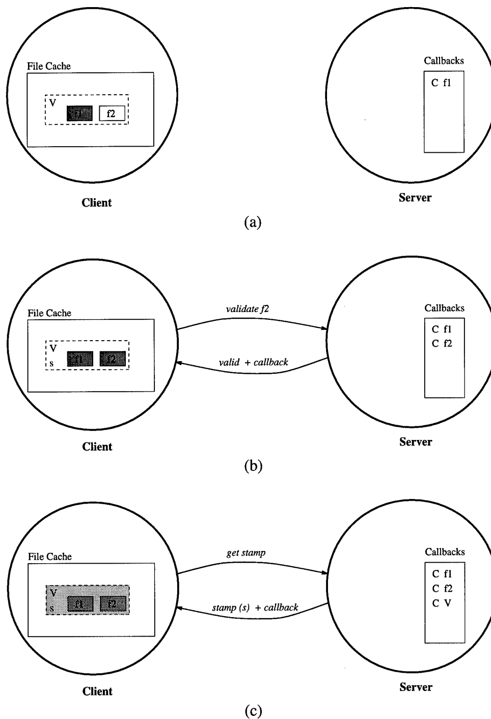
Figure 4.1: Obtaining a Volume Callback
