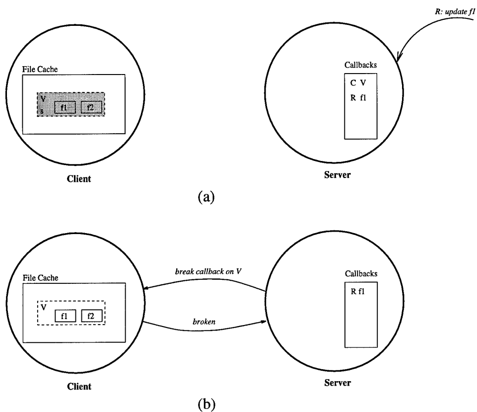
Figure 4.3: Breaking a Volume Callback
