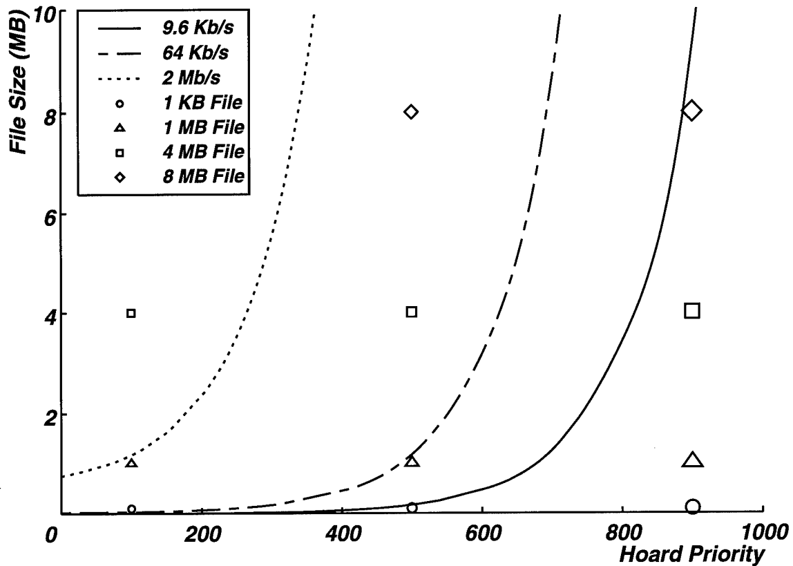
Figure 6.8: Patience Threshold versus Hoard Priority
