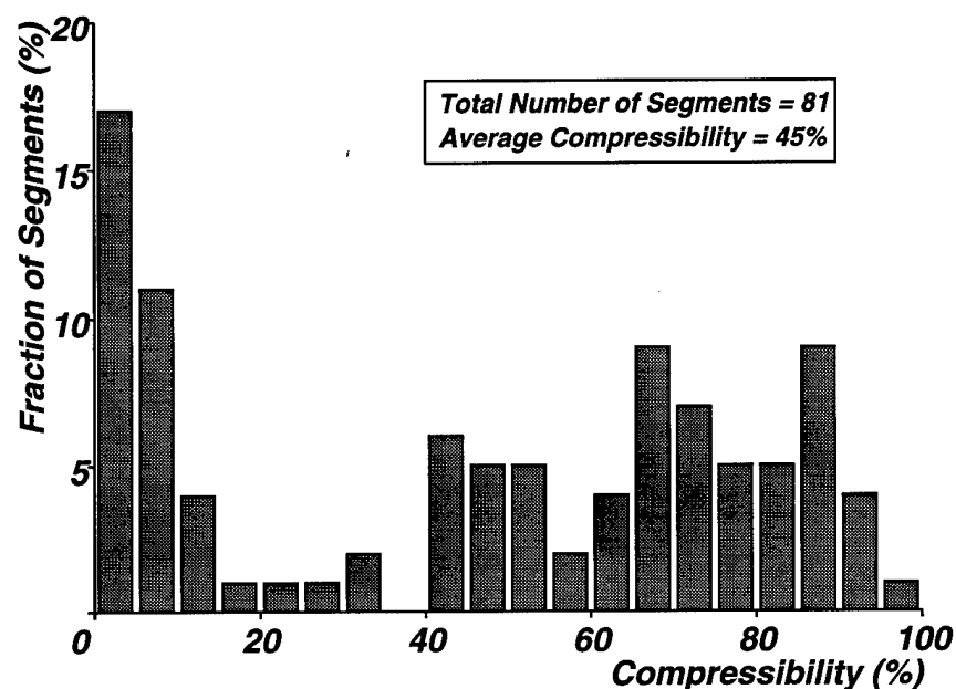
Figure 7.13: Compressibility of Trace Segments
