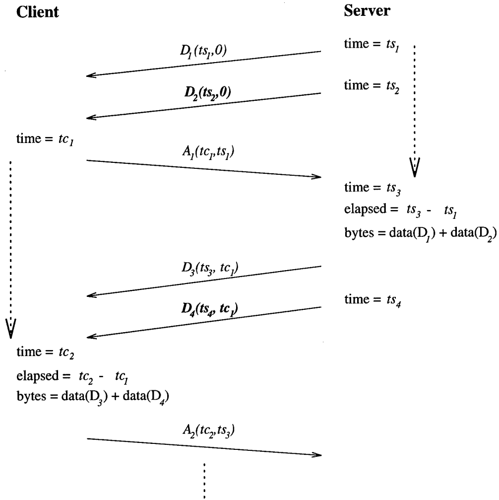
Figure 3.10: Measuring SFTP Rounds
