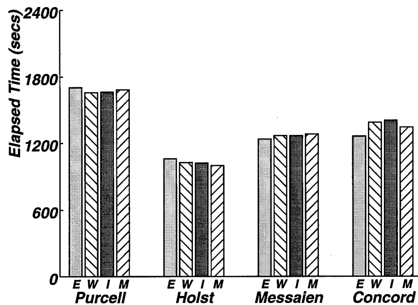
Figure 7.22: Performance of Trace Replay ( \lambda = 10 seconds, A = 600 seconds)
