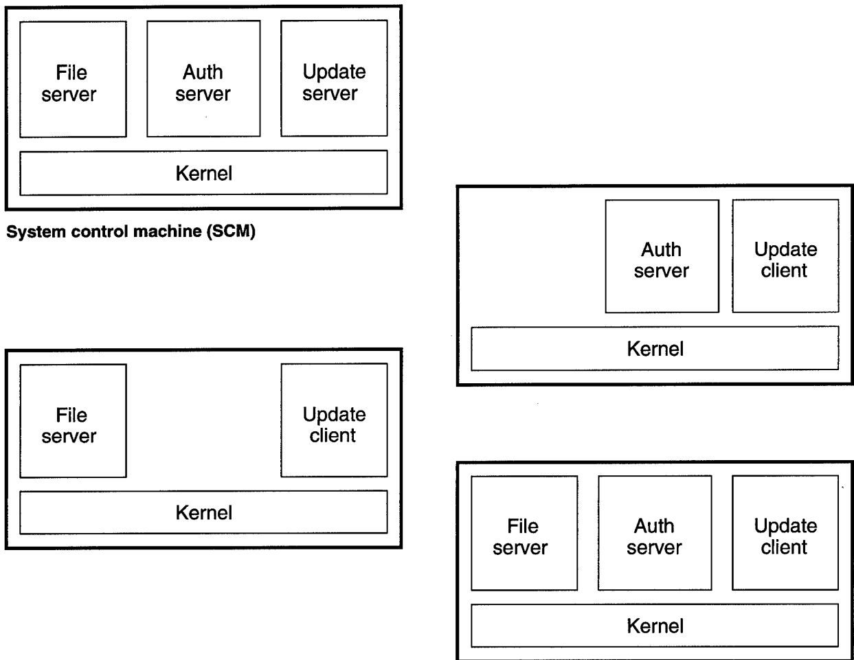
Figure 2.10: Coda Server Structure
