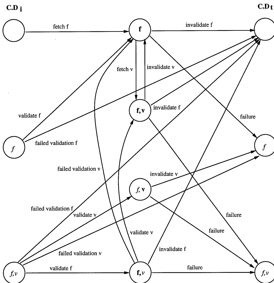
Figure A.1: Client State Transitions – Invalidation Based, Large Granularity
