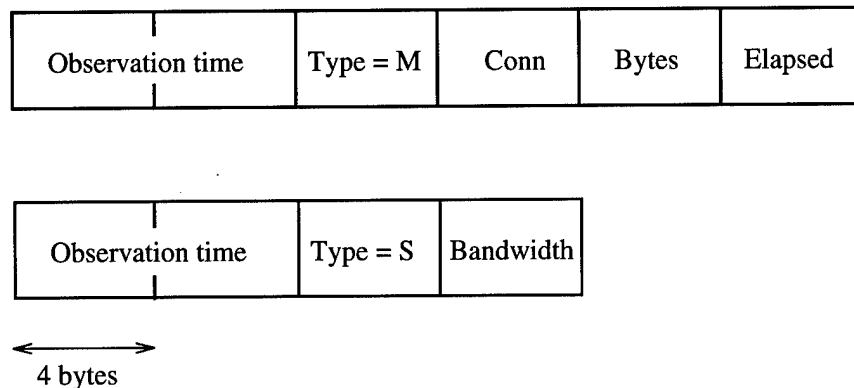
Figure 3.8: Transmission Log Record Formats
