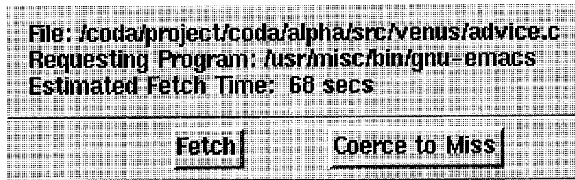
Figure 6.3: Weakly Connected Miss
