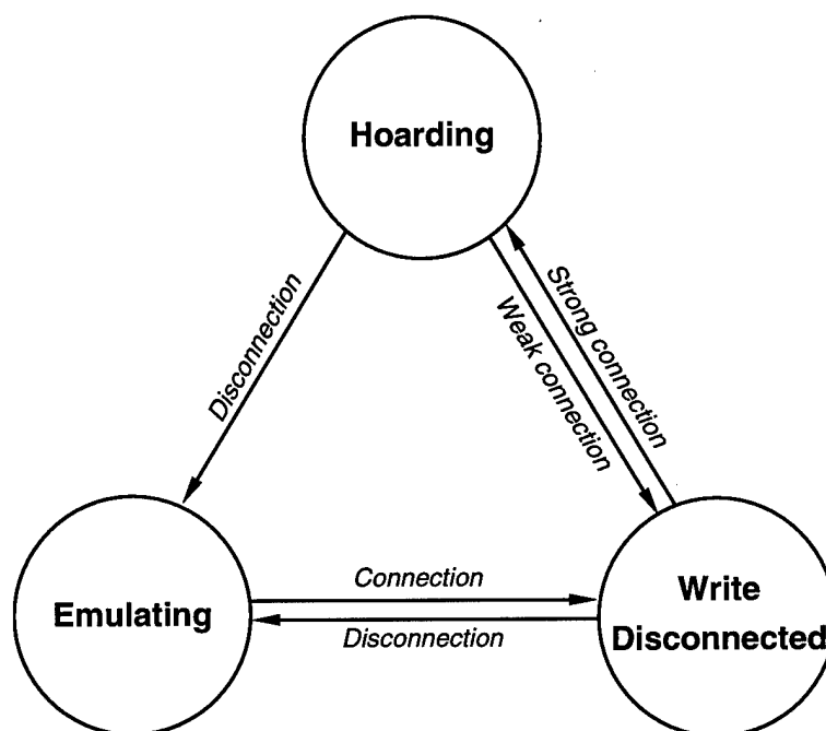
Figure 5.1: Venus State Transition Diagram
