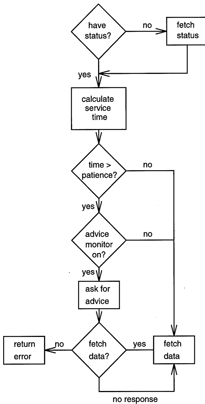
Figure 6.4: Cache Miss Handling
