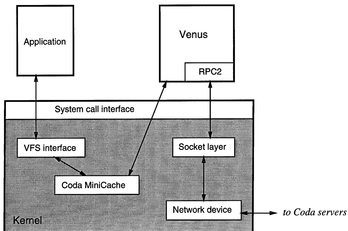
Figure 2.9: Coda Client Structure
