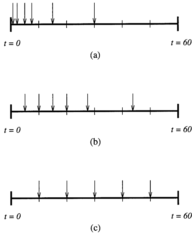
Figure 3.2: RPC2 Retransmission Intervals
