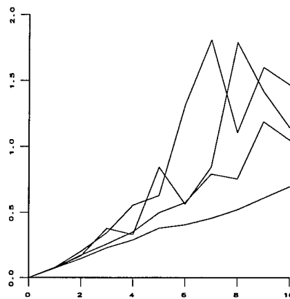
Graph 1 : 3D error for Euclidean reconstruction (near points). This graph shows all methods. All perform almost equally. Marginally the best results are given by Mid-point, Linear-LS and Iterative-LS, which are almost indistinguishable. The Polynomial method performs marginally worse than the others. It is designed to minimize 2D error, which explains why optimal in this regard, it is not quite optimal for 3D errors. Euclidean reconstruction is the only instance in which Mid-point performed even marginally well, and the only case in which Polynomial and Poly-Abs were beaten.
