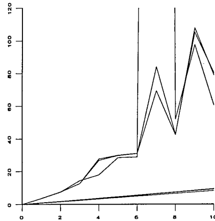
Graph 3 : 2D error for Euclidean reconstruction (near points) The configuration is the same as for Graph 1 , except that the average (not RMS) 2D error is measured. Of course Poly-Abs performs best (since it is optimized for this task) but Polynomial, Iterative-LS and Iterative-Eigen are almost indistinguishable. The three very bad performers are Linear-Eigen, Linear-LS and Mid-Point. The maximum Y-scale is 120 pixels. This graph shows that 2D error and 3D error are not well correlated, since despite large 2D errors, these methods perform well in terms of 3D error.
