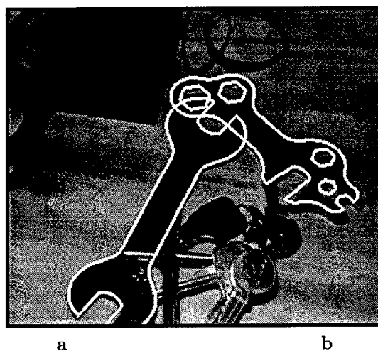
Figure 7.5: Single concavities are sufficient to recognise the two model instances shown in (b). The redundancy of the canonical frame representation gives much better tolerance to occlusion than global shape methods. The left hand object gained 67.1% boundary support, and the right object 81.6%.
