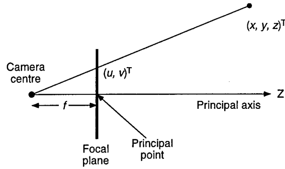
Figure 1.1: Pinhole camera geometry
