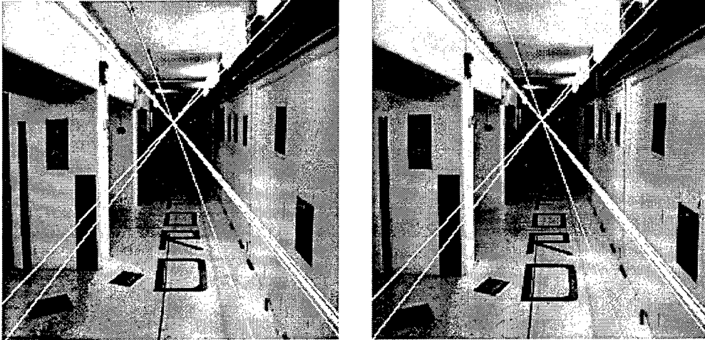
Figure 2.4: Corridor Scene In the corridor scene the epipoles are right in the image.
