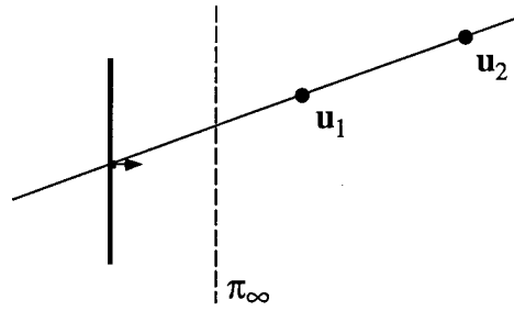
Figure 4.9: Which points are in front. In the reconstruction shown, point u_1 is closer to the third camera than u_2 . If, however, we apply an orientation-reversing projective transformation that maps the plane \pi_\infty to infinity, then the two points will still lie in front of both cameras, but now point u_2 will lie closer to the third camera. This is because locally the front and back of the cameras will be reversed by the orientation-reversing transformation. In order to reach u_1 from the centre of the third camera, without crossing \pi_\infty it is necessary to pass through u_2 first.
