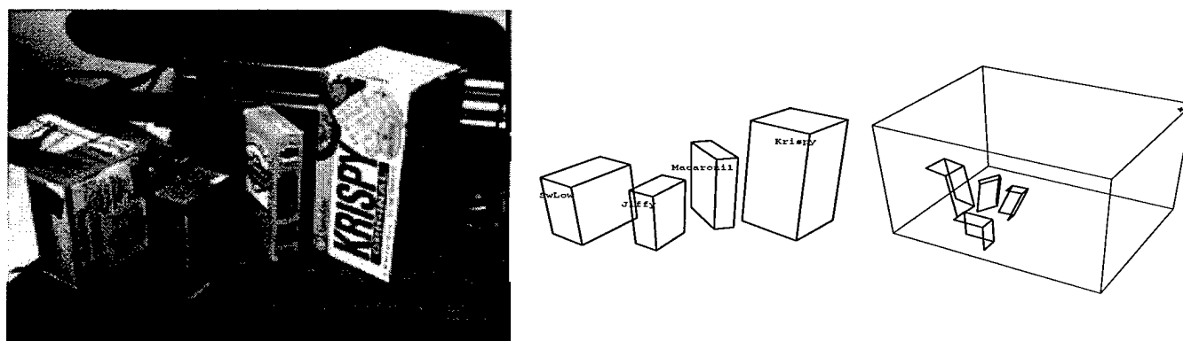
Figure 7.21: (a) A scene containing polyhedra all of which are projectively equivalent, but Euclidean inequivalent. (b) A labelling of the scene. (c) A Euclidean reconstruction of the polyhedral world shown in (a). The optical centre is the marked point in the top right-hand corner of the figure.
