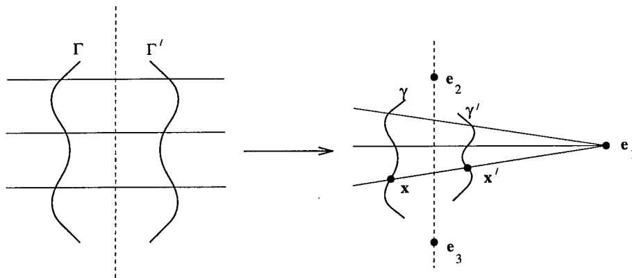
Figure 7.14: The profile of a surface of revolution is projectively equivalent to two curves with bilateral symmetry. Under a projective transformation parallel correspondences (left) converge to a vanishing point (right). Corresponding points \mathbf{x} \leftrightarrow \mathbf{x}' are related in this case by a particular plane projective transformation, T , called a planar harmonic homology. The transformation has a line of fixed points, the image of the axis of symmetry, which result from two of the eigenvalues of T being equal. There is also a fixed point, \mathbf{e}_1 , not on the line, called the centre of the homology which defines correspondences between symmetrical points on each side of the contour. That is, corresponding point pairs and the centre of the homology are collinear. The cross-ratio of \mathbf{e}_1 , the corresponding points \mathbf{x}, \mathbf{x}' , and the intersection of their join with the axis, is harmonic. (The line of fixed points is \mathbf{e}_2 \times \mathbf{e}_3 , where \mathbf{e}_2 and \mathbf{e}_3 are the eigenvectors with equal eigenvalues. The third eigenvector, \mathbf{e}_1 , is distinct and non-zero, and is the centre for a pencil of fixed lines.)
