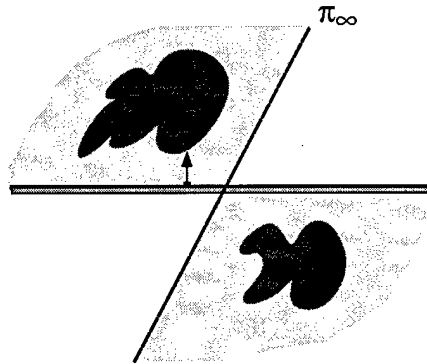
Figure 4.2: Effect of a projective transform with positive determinant. The principal plane of the camera and the plane \pi_\infty divide R^3 into four segments. One pair of opposite segments (shown shaded) are transformed to points in front of the camera. The opposite pair of segments are transformed to points behind the camera. In the local neighbourhood of the camera centre the front and back of the camera are preserved. This consideration determines which pair of segments become the front of the camera. Thus the two dark shaded sets of points lie in front of the camera after transformation. For a transform with negative determinant the opposite pair of segments become the front of the camera.
