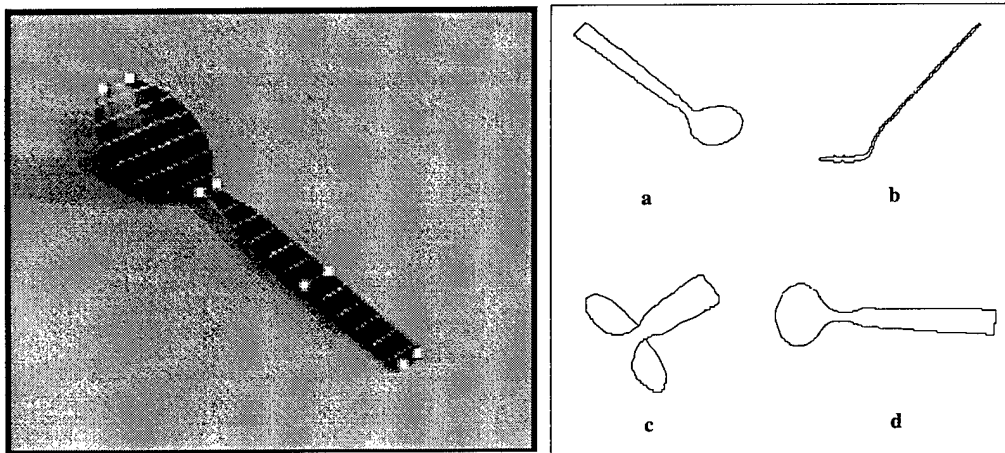
Figure 7.12: A single view of an object with a plane of bilateral symmetry, such as a teaspoon, is sufficient to allow a full 3D projective reconstruction. Only two pairs of distinguished points are needed for the approach, these are recovered from surface markings and can be used to determine the epipolar structure of the image. Using this epipolar structure an arbitrary number of correspondences can be produced. Four different views are shown of the 3D reconstruction computed from the image. The construction works very well: note the planarity of the handle recovered in (b), and the full 3D shape in all of the images.
