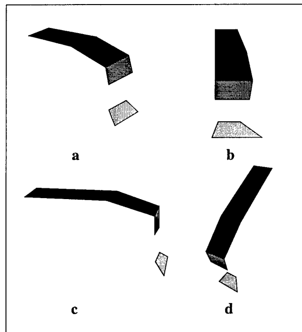
Figure 7.11: Three dimensional structure is recovered, modulo a projectivity, from the single view of the points marked on the stapler in figure 7.10b. Four typical views are shown with only (a) at a viewpoint close to that of the original image. Note the collinearity of the line segments in (b), this demonstrates the accuracy of the recovered structure.
