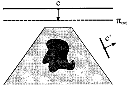
Figure 4.6: Second camera in front of the first camera We can separate the two camera centres c and c' with a plane \pi_\infty lying just in front of the principal plane of the first camera. The point set X lies entirely inside the truncated cone (lightly shaded). The plane \pi_\infty can be chosen sufficiently close to c so as not to meet this cone. Consequently, it will not separate the point set X .
