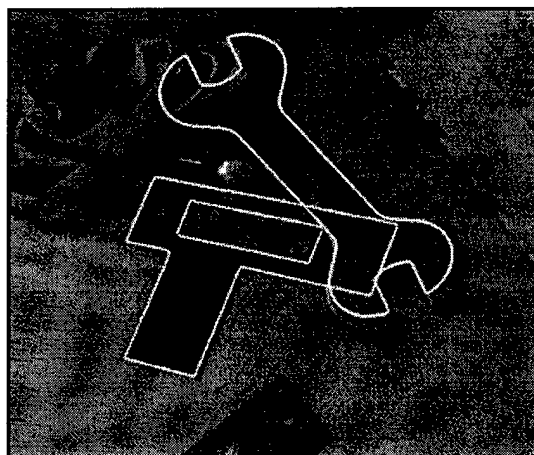
Figure 7.6: A demonstration that both types of invariant index can be used to recognise objects in a single image. The bracket is indexed using algebraic invariants and the spanner is indexed using the canonical frame signature.
