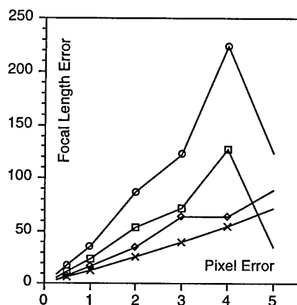
Figure 6.3: Error in estimation of focal length. The plot shows the standard deviation in the estimate of focal length at different noise levels. In all cases, the mean estimated focal length was close to 400 (the correct value). The four plots show the standard deviation for values of \alpha equal to (from the top) 20, 39, 58 and 75 pixels. Thus, in most cases, for noise levels less than 2 pixels, the estimated focal length lies in the range between 350 and 450. The apparent improvement in performance for pixel errors of 5 pixels in the top two plots is due to the fact that the algorithm failed for a substantial percentage of such tests, which were therefore not included in this statistic.
