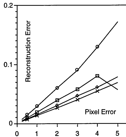
Figure 6.5: Reconstruction Error. This graph shows the RMS reconstruction error for different noise levels and the same values of \alpha as before. The vertical axis gives the absolute RMS reconstruction error in length units where the reconstructed set of points has radius about 1.5 units.
