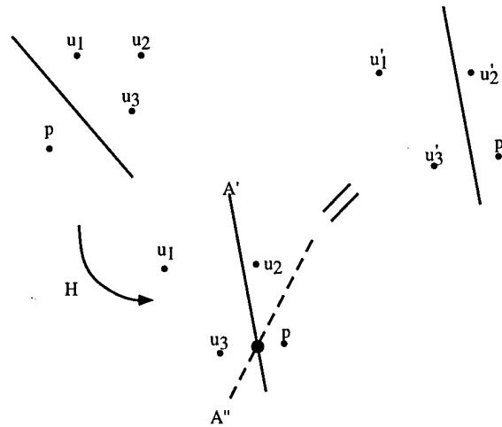
Figure 3.1: Intersection of a line with a plane defined by three points. Consider points u_1, u_2, u_3 and the epipole p in one image and corresponding points u'_1, u'_2, u'_3 and p' in the second image. Compute the 2D projective mapping H that takes the points to their corresponding points in the second image. Transfer the line by H and compute its intersection with the line in the second image. This intersection point is the point where the line meets the plane of the three points, as seen in the second image.
