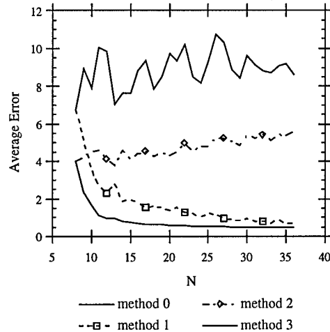
Graph 2 : Effect of normalization on the two stages of the algorithm.
