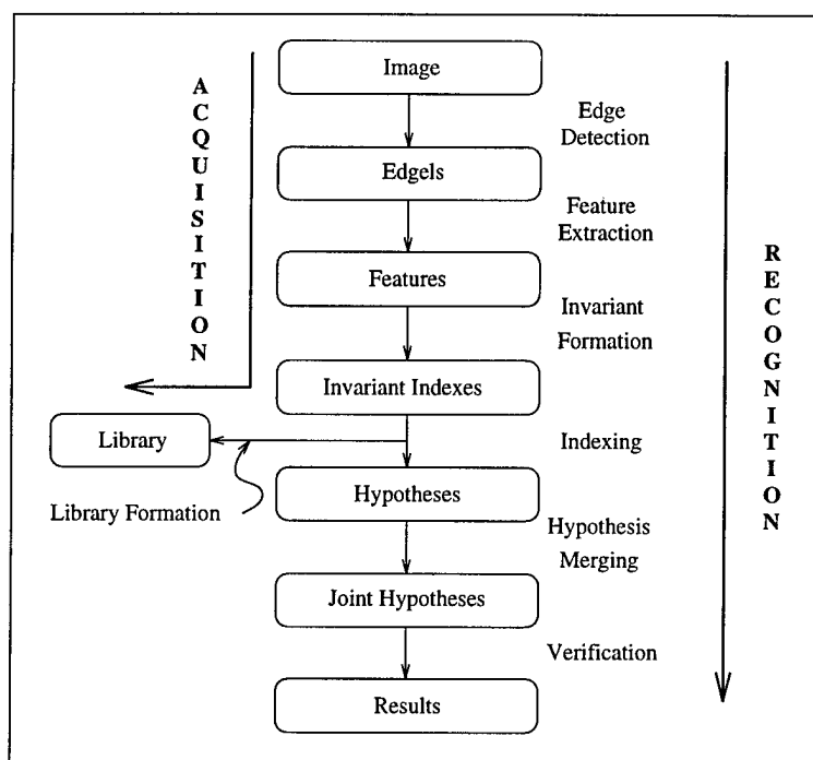
Figure 7.2: The recognition system has a single grey scale image as input and the outputs are verified hypotheses with associated confidence values. Many of the processes are shared by the acquisition and the recognition paths. The recognition system is similar to previous systems [39] in all but the indexing and hypothesis merging stages.
