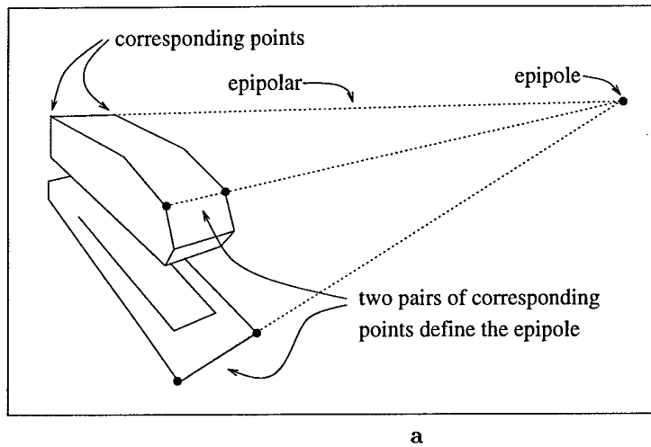
Figure 7.10: (a) The epipole can be located using the intersection of lines between two corresponding points on a bilaterally symmetric object (the points are marked by solid circles). Epipolars can then be constructed through the epipole to aid correspondence. (b) Typical corresponding points determined in this manner.
