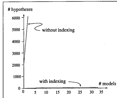
Figure 7.7: The number of hypotheses that have to be verified as the number of models in the library is varied. The results show an average over fifty scenes containing only one object in the library, but with other clutter and occlusion present. Over 2000 indexes are created for the scene, which corresponds to the number of hypotheses that would have to be verified per model feature group if alignment is used. Therefore, there is a rapid linear growth in the number of hypotheses created as the model base is expanded. However, the number of hypotheses created through indexing remains substantially lower — there is a linear growth, but with a very low constant of proportionality.
