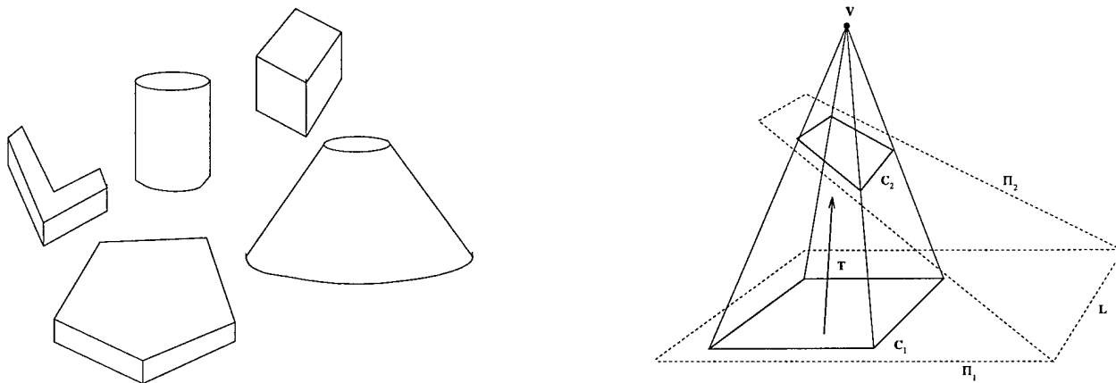
Figure 7.20: An extruded surface is a section cut from a general cone by two planes. (a) A range of examples of extruded surfaces; note that for most examples, the vertex is at infinity. (b) The top and base image curves, C_1 and C_2 , of an extruded surface are related by a particular projective transformation T , called a planar homology. Corresponding points lie on lines through V , which is the fixed point of the transformation (the centre or vertex). The line L , which is the image of the intersection of the two planes that cut the "cone", is a line of fixed points of the transformation (the axis).
