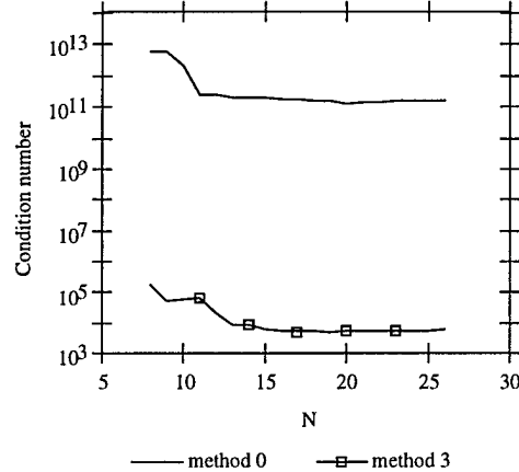
Graph 1 : Effect of Normalization on the Condition Number.
