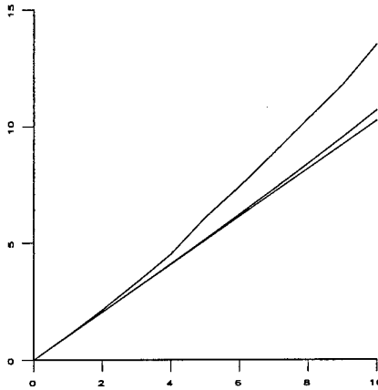
Graph 9 : Affine Invariance. The three curves shown are from the bottom Iterative-Eigen (Euclidean) Iterative-LS (Euclidean and Affine superimposed) and Iterative-Eigen (Affine). Thus, as predicted by theory, the Iterative-LS method is precisely affine-invariant, but Iterative-Eigen is not (but almost). Once more we remark that except for occasional non-convergence, these would be good methods.
