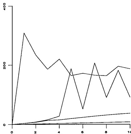
Graph 5 : 2D error for Projective reconstruction (near points) . This is the case for which all methods performed well in the Euclidean case. This graph shows the results for methods (from the bottom) Polynomial, Iterative-Eigen, and Iterative-LS. The method Poly-Abs (not shown) performed almost identically with Polynomial. This graph shows that Polynomial, or Poly-Abs is the best method for projective reconstruction, whereas Iterative-Eigen and Iterative-LS (except for occasional non-convergence) perform almost as well. Full Y-scale is 20 pixels.
