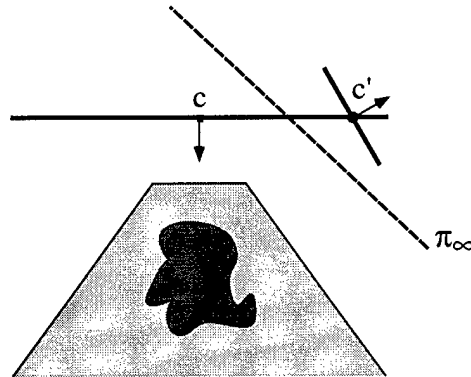
Figure 4.7: Second camera lies on the principal plane of the first camera. We can separate the two camera centres c and c' with an oblique plane \pi_\infty which crosses the principal plane of the first camera. Plane \pi_\infty can be chosen so as not to meet the cone containing X , and consequently will not separate X .
