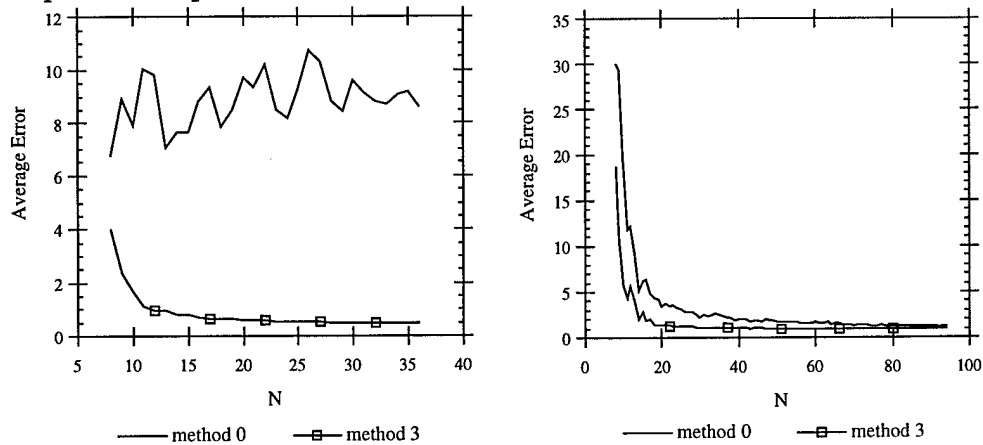
Graph 3 : Comparison of normalized and unnormalized 8-point algorithms.
