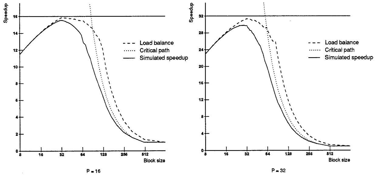
Figure 11: Performance bound for parallel dense Cholesky factorization, n = 1000 . T_{op}(1) = 5 , \beta = 4 .
