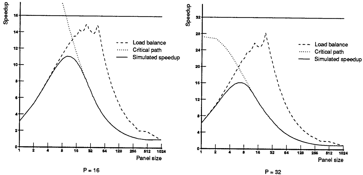
Figure 5: Performance and performance bounds for panel-oriented parallel dense Cholesky factorization, n = 1000 . T_{op}(1) = 5 , \beta = 4 .
