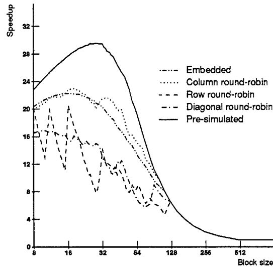
Figure 13: Performance results for five block mapping strategies. n = 1000 , T_{op}(1) = 5 , \beta = 4 , P = 32 .
