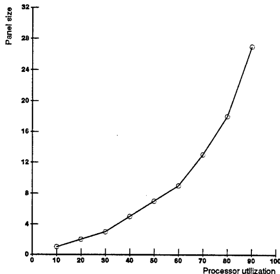
Figure 7: Optimal panel sizes at various processor utilization levels.
