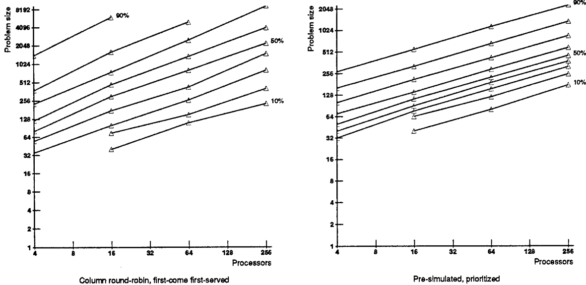
Figure 14: Problem sizes necessary to achieve different processor utilization levels.
