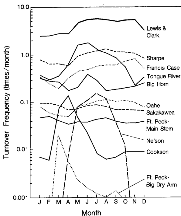
Fig. 9. Turnover frequencies of Missouri River Basin reservoirs. Data for the Big Dry Arm of Lake Fort Peck are based on the assumption that this arm acts as an independent water body. Monthly data represent averages over the periods for which records have been kept.
