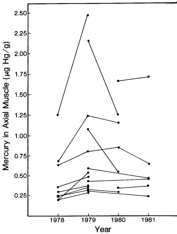
Fig. 14. Mercury concentration (wet weight) in individual northern pike in the Tongue River Reservoir, biopsied and analyzed for mercury (wet weight) at least twice between spring 1978 and spring 1981.
