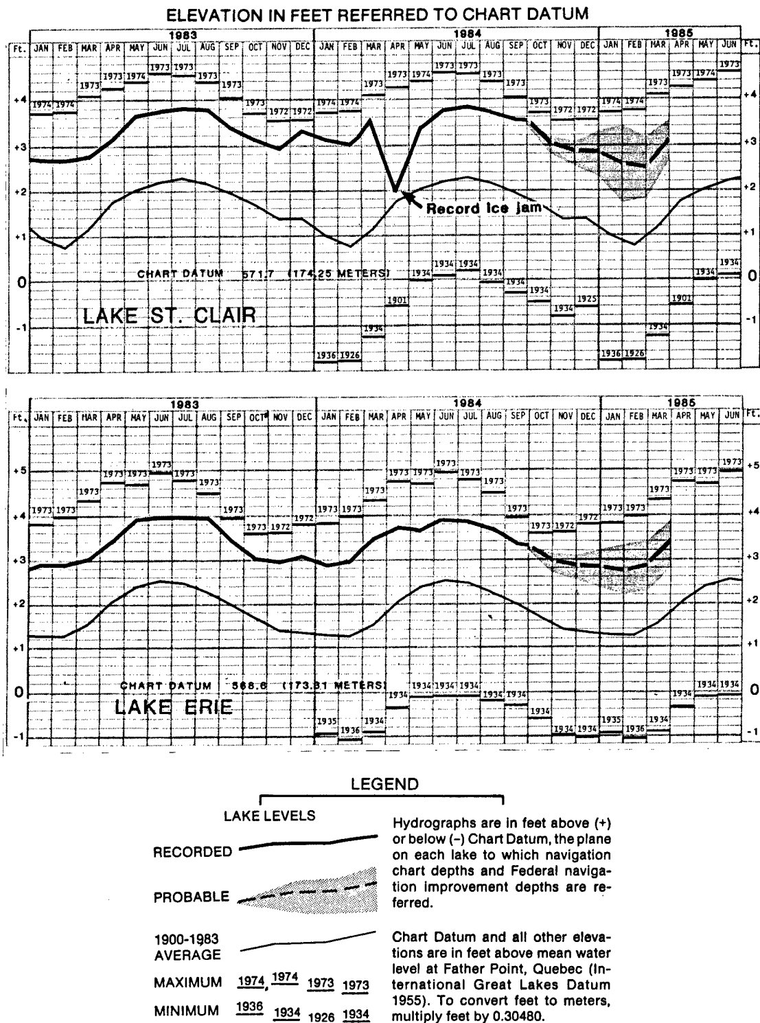
Figure 18. Hydrograph of Lake St. Clair and Lake Erie water levels, showing the impact of a record ice jam in the St. Clair Delta in March and April 1984 (U.S. Army Corps of Engineers). Note the slight dip in Lake Erie water levels in May in response to the St. Clair Delta ice jam.
