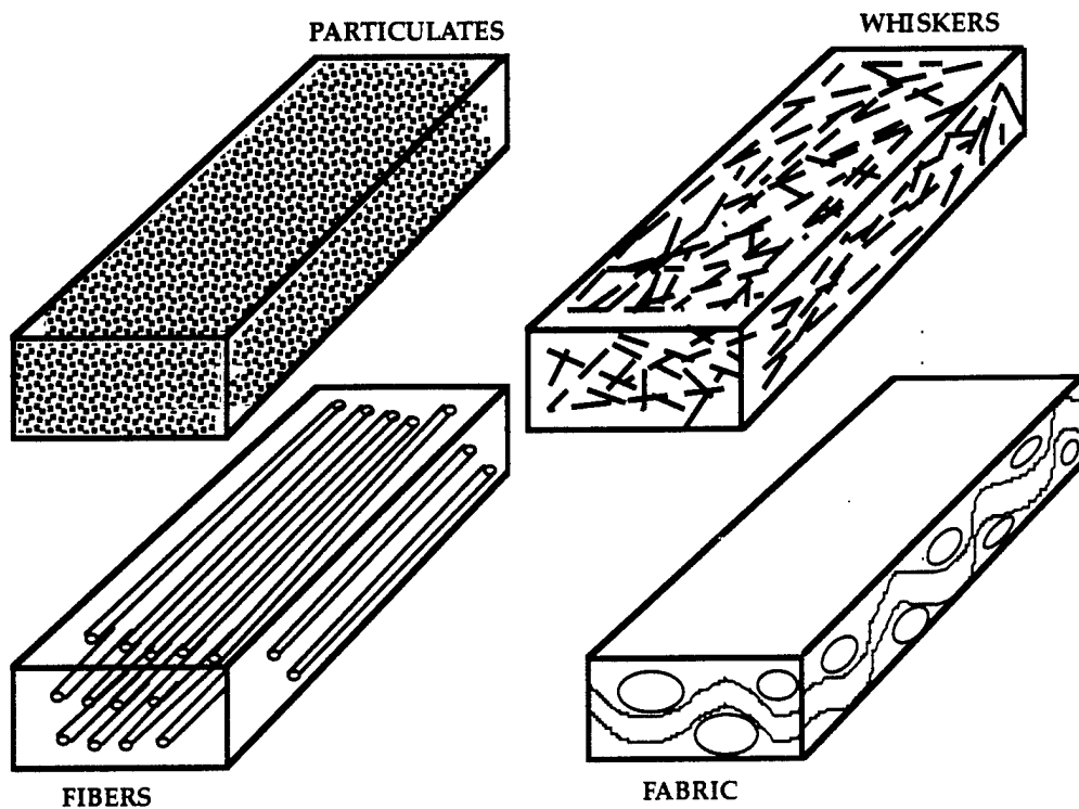
Figure 6-3. Reinforcement Types
