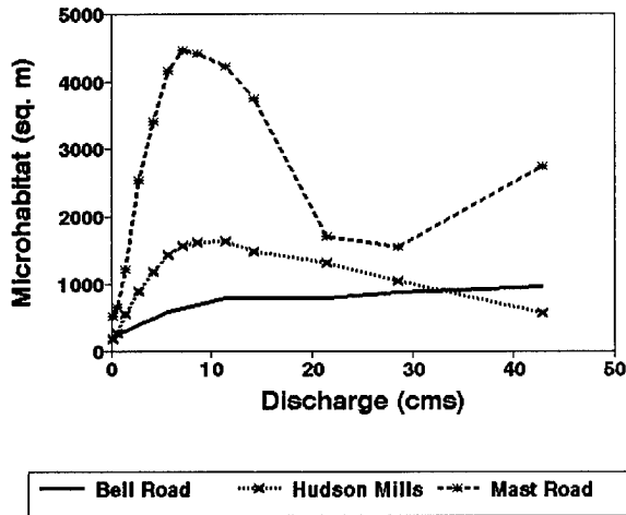
Fig. B10. Usable microhabitat versus discharge for young-of-year rock bass, summer daytime hours.
