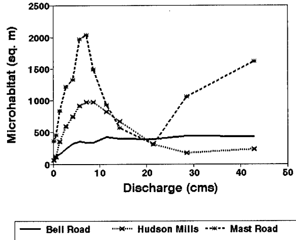
Fig. B11. Optimal microhabitat versus discharge for young-of-year rock bass, summer nighttime hours.
