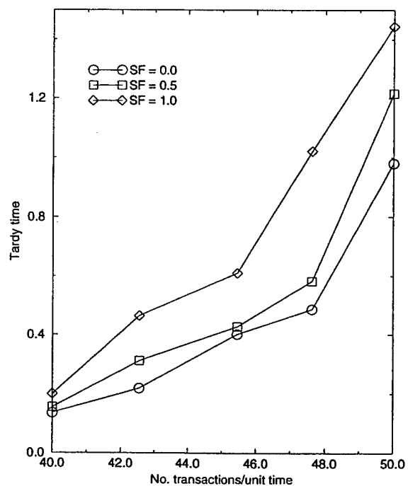
Figure 5.2: Adaptive 2PL - Tardy Time
