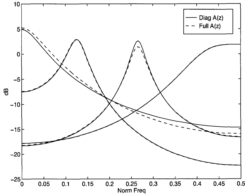
Figure 14. Estimated Markov-modulated vector AR(2) spectrum using both a diagonal and full predictors.
