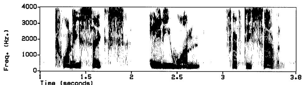
Figure 4. Spectrogram of YOHO combination lock phrase, "Forty One, Sixty Nine, Fifty Six".
