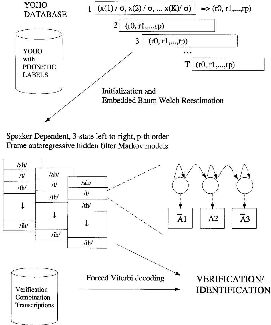
Figure 19. The phoneme frame autoregressive hidden filter approach models individual phonemes as 3-state left-to-right hidden filters. The \bar{A} denotes a p -order hidden filter, as reestimated in Section 3.4.
