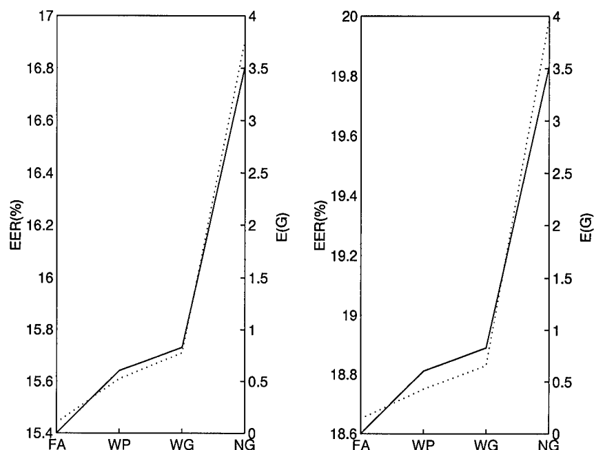
Figure 27. Equal error rates (Dashed) for males (left) and females (right) over the YOHO database with one combination per test trial. Also shown is Entropy (Solid) in bits/phoneme of the language induced by the grammar.
