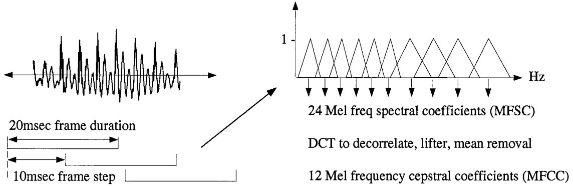
Figure 5. Typical Speech Processing/ Feature extraction.
