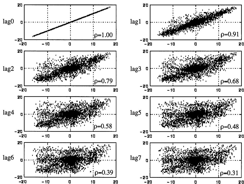
Figure 6. Scatterplot of first cepstral coefficient c_1(t) for lags 0-7. Each point within a subplot is the order pair (c_1(t), c_1(t + l)) where l is lag. Inset within each subplot is the correlation coefficient over all data.
