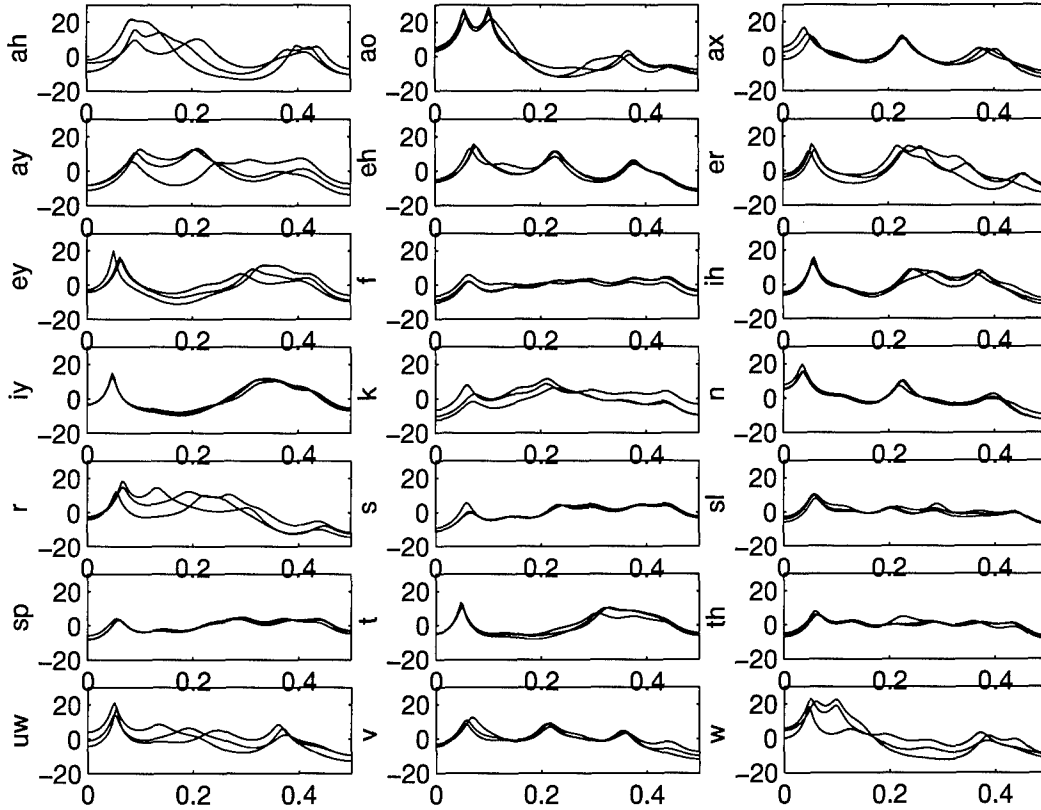
Figure 12. Extended Poritz Method for Temporal Phoneme Modeling of YOHO Speaker. Each speaker is represented by 21 3-state left-to-right monophone models. Shown for one speaker, the power spectrum of the resulting filter estimates for all models and all states.
