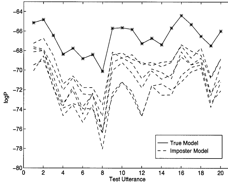
Figure 21. Typical log-likelihood of true model and imposter models shows the variability based on the transcription (prompted words) which forces some non-fixed thresholding scheme.
