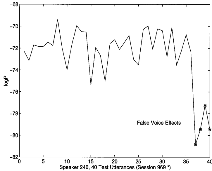
Figure 20. False voice effects of speaker 240, session 969, shown in the forced Viterbi normalized log-likelihood scores (*).
