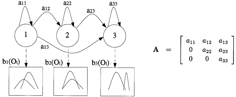
Figure 1. Standard three state left-to-right multivariate Gaussian mixture hidden Markov model. Shown with upper triangular transition matrix \mathbf{A} . Each state is described by a parametric output density b_i(O_t) .
