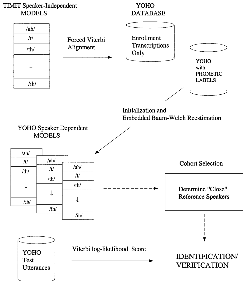
Figure 17. Speaker recognition system overview.
