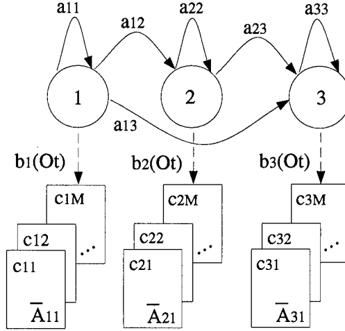
Figure 2. Juang's frame autoregressive mixture extensions to the Poritz hidden filter. While Poritz proposed single filter states, Juang extended to multiple mixtures.
