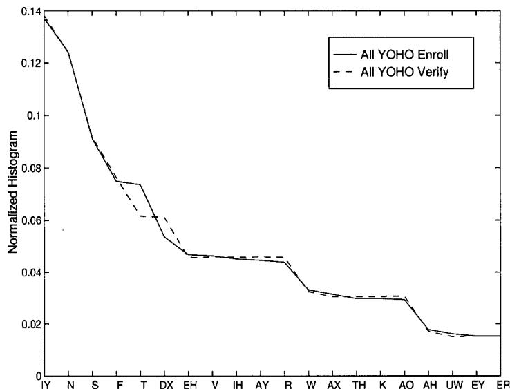
Figure 18. Histogram of all YOHO enrollment and verification utterances, after a forced Viterbi segmentation bootstrapped from TIMIT.
