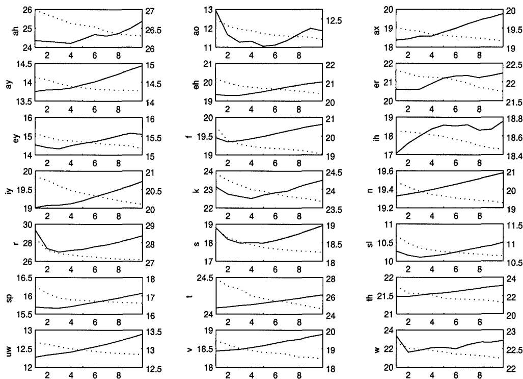
Figure 26. Akaike Information Criterion (AIC) for Vector Phoneme Models By Examining the Diagonal Covariance at Several Order Models. The subplots show each of the 21 monophone models' MLE of the average noise variance (dashed line). Note this MLE decreases with increasing model order and the AIC (solid line) acts accordingly, decreasing to a minimum, then increasing.
