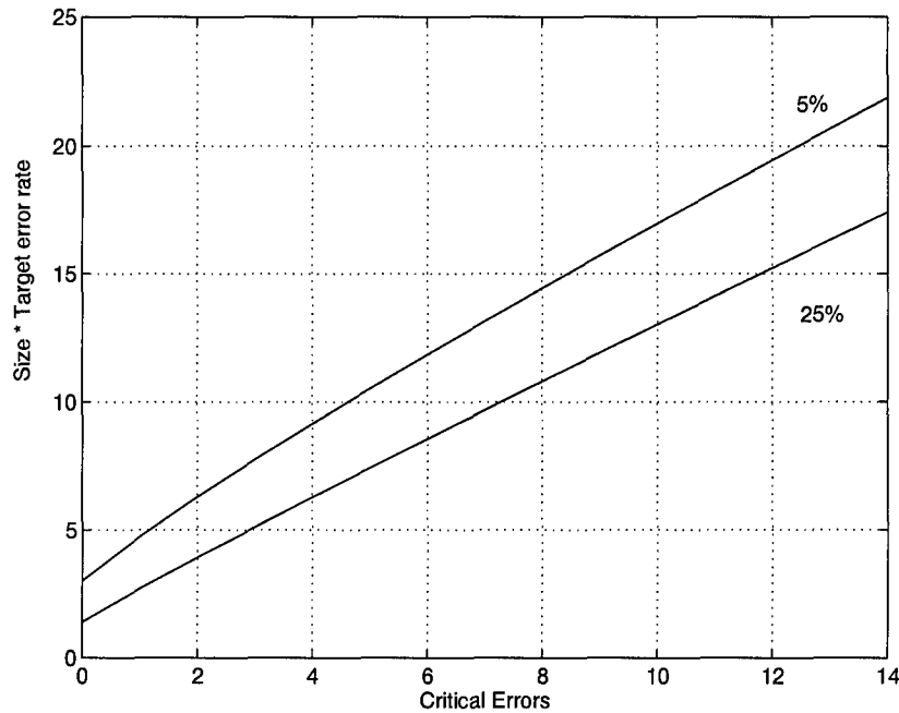
Figure 23. Critical Errors for Tests Designed at the 5% and 25%. The curve is generated by searching for the appropriate \lambda value given a particular (discrete) Critical Error. The curve is used by knowing \lambda = N \cdot Ter , the Target Error Rate ( Ter ) and the size of the database N , then reading over and down.
