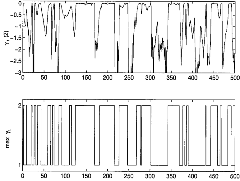
Figure 8. Uncovering the AR Hidden State Sequence. Shown are the actual state log likelihood \gamma_t(2) and the most likely state sequence \max_i \gamma_t(i) for the process described in Figure 7.
