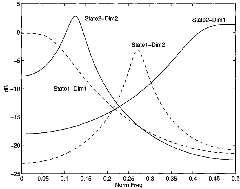
Figure 13. Markov-Modulated Vector AR(2) process.
