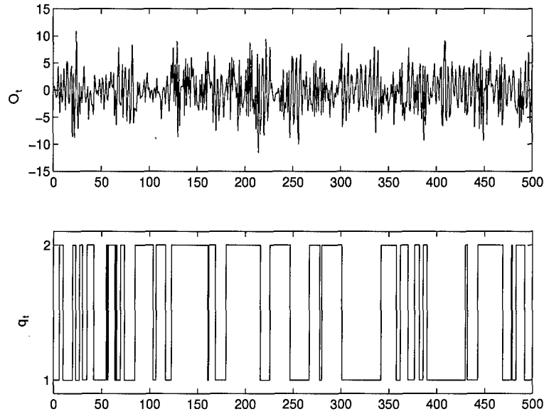
Figure 7. Sample AR(2) Markov-Modulated Source with Actual State Sequence.
