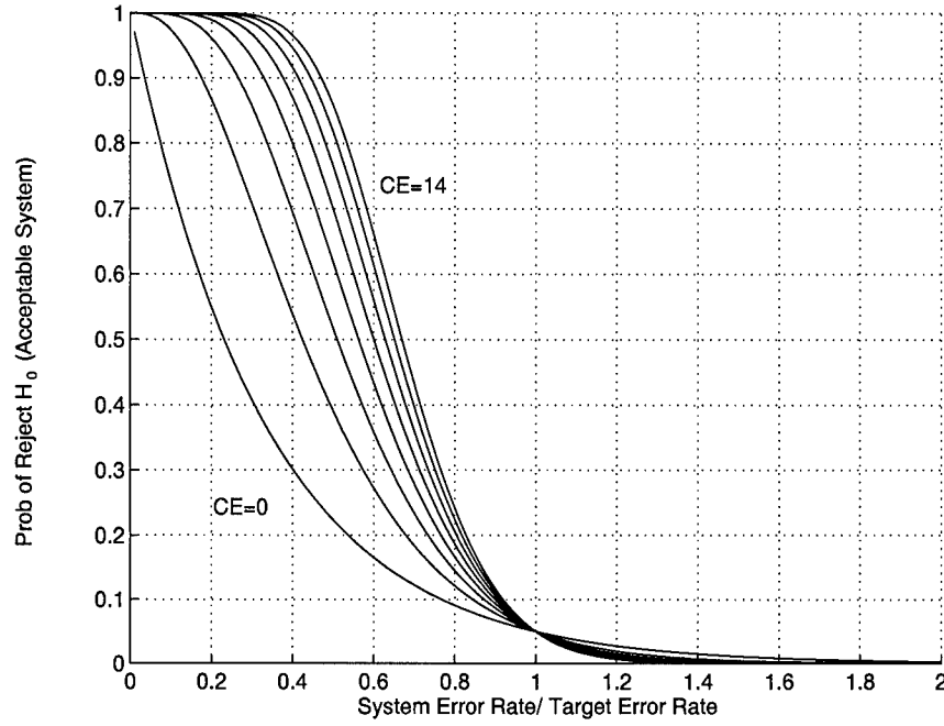
Figure 24. Probability of Rejecting H_0 - Accepting the System Meets the Target Error Rate Ter , for number of critical errors (0,2,4,6,8,10,12,and 14) at the 5% significance level.
