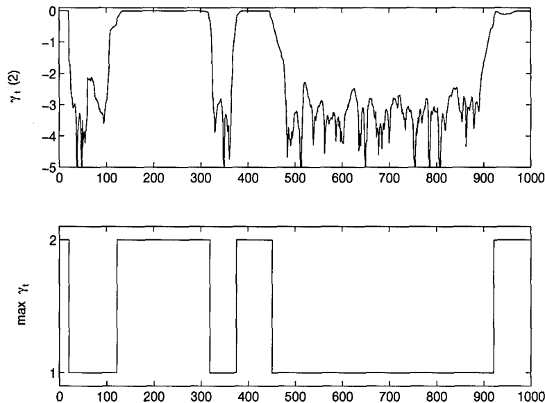
Figure 10. Uncovering the ARMA Hidden State Sequence. Shown are the actual likelihoods \gamma_t(2) and the most likely state sequence \max_i \gamma_t(i) for the process described in Figure 9.
