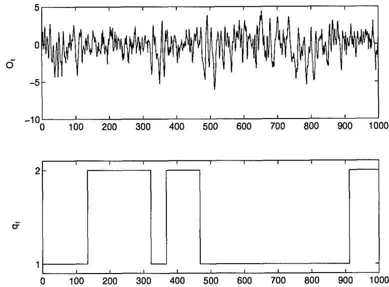
Figure 9. Markov-Modulated ARMA(2,2) Process
