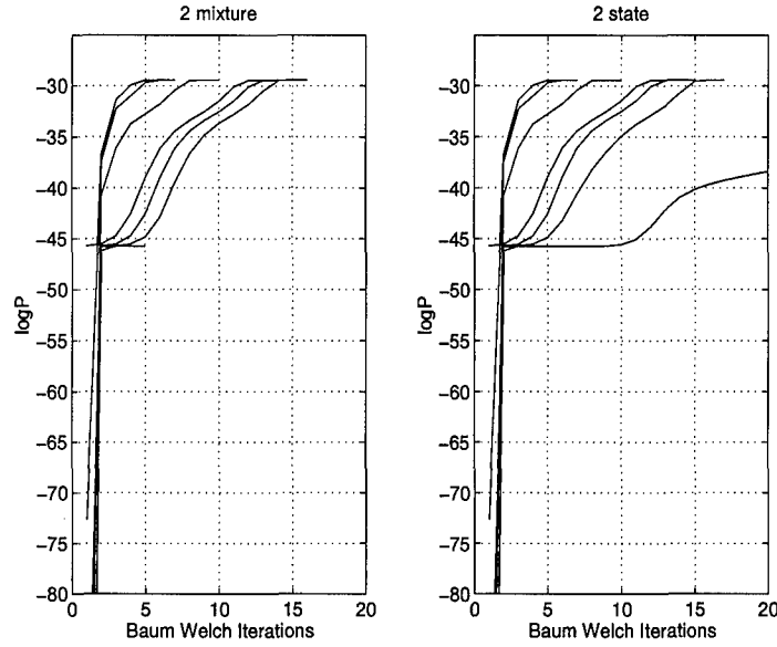
Figure 16. Learning the maximum likelihood models from 10 random starts based on the architectures of the original HMM \lambda (2 mixture) and theoretical equivalence model \lambda_E (2 state). Almost all models converged to the same equivalent log-likelihood value of -29.45 .
