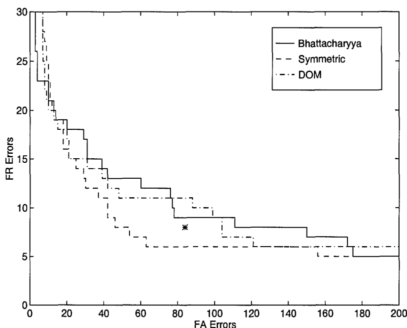
Figure 25. Speaker Verification False Accept and False Reject Error (#) using DOM, Bhattacharyya and Symmetric cohort selection strategies. Results show the effect of an unseen threshold. Data only used male speakers, when prompted with 4 combination lock phrases and normalized with 10 cohorts using full 39-dimensional features (MFCC+E+ \Delta + \Delta\Delta ).
