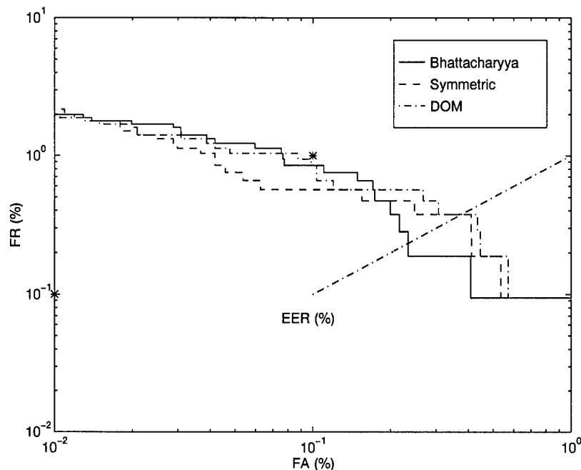
Figure 22. Speaker Verification False Accept and False Reject Error Rates (%) using DOM, Bhattacharyya and Symmetric cohort selection strategies. Results show the effect of an unseen threshold. Data only used male speakers, when prompted with 4 combination lock phrases and normalized with 10 cohorts using full 39-dimensional features (MFCC+E+ \Delta + \Delta\Delta ). Best Equal Error Rate shown is 0.21% using the Bhattacharyya normalization. Note: (*) denotes U.S. Government requirement of 1% FR and 0.1% FA [18, 17].
