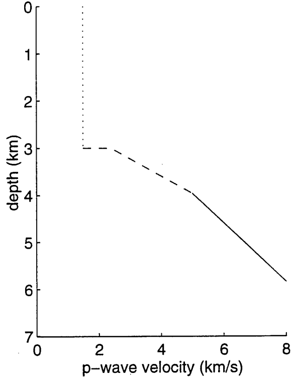
Velocity Structure
