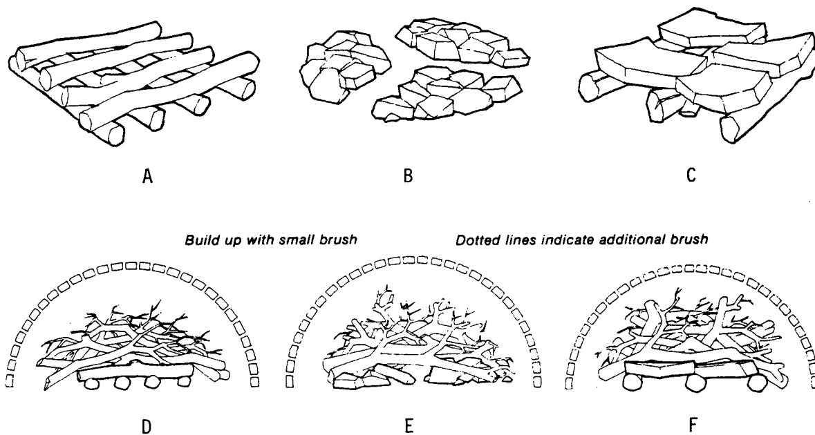
Figure 3.3-22. Construction of brush pile shelters demonstrating base construction methods and construction with dead brush (D-F) (A-Logs, B-Boulders, C-Log/Boulder Combination) (from Gutiérrez et al. 1979).
