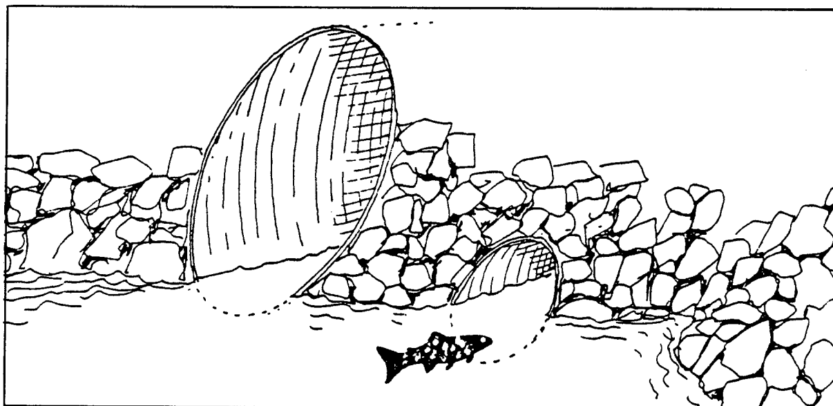
Figure 3.1-6. The arch culvert provides for fish passage (from Nelson et al. 1978).
