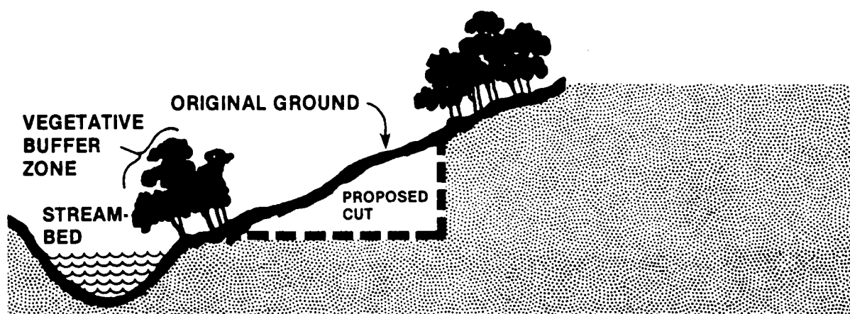
Figure 3.2-1. Vegetative buffer zones to protect stream water quality (after U.S. Environmental Protection Agency 1976).
