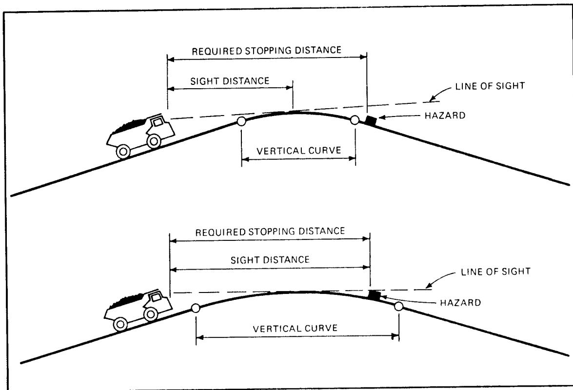
Figure 3.1-1. Sight distance on vertical curves (from Chironis 1978).
