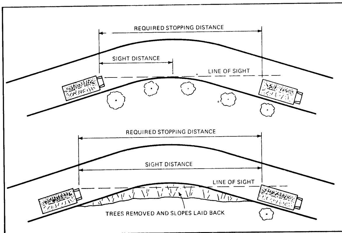
Figure 3.1-2. Sight distance on horizontal curves (from Chironis 1978).
