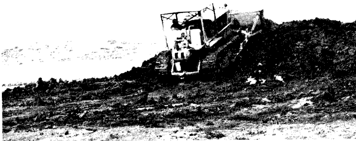
Figure 3.3-10. Earthen-mound islands can easily be constructed with a bulldozer during impoundment construction (Jones 1975).
