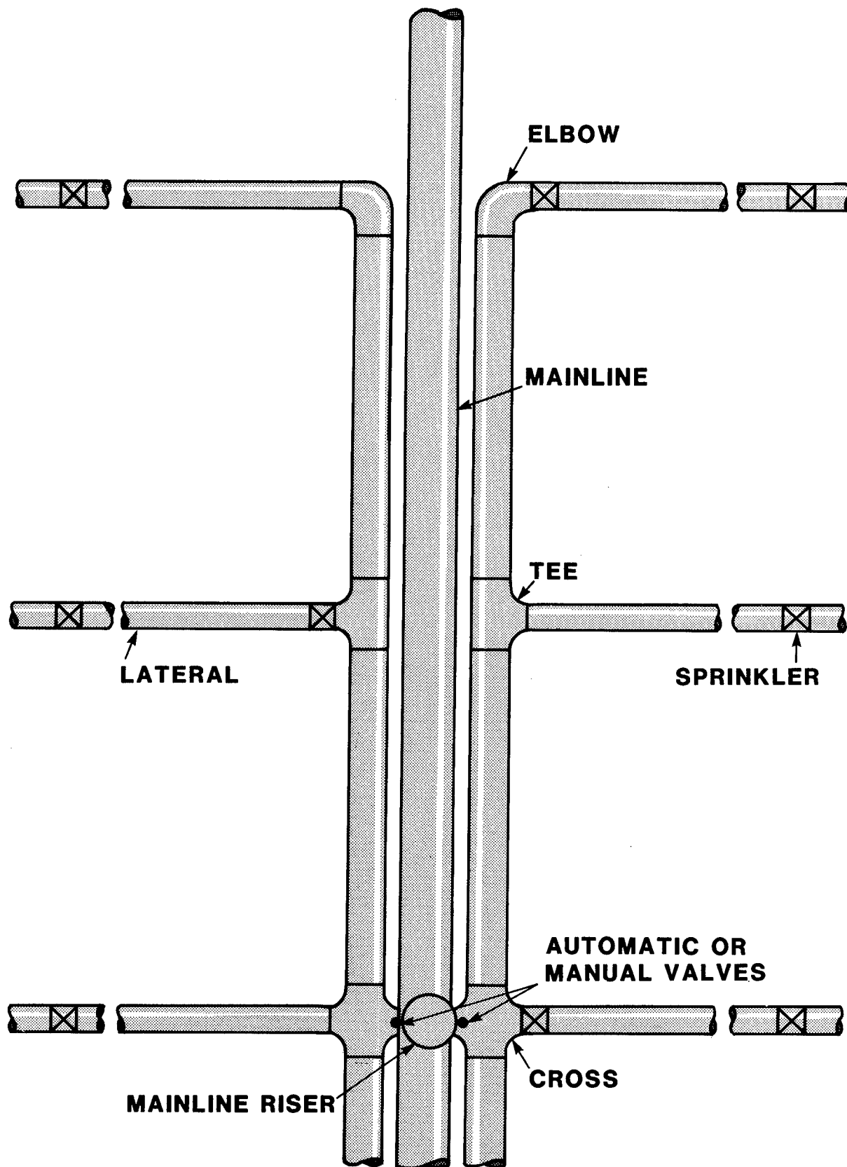
Figure 3.3-4. Manifold detail.
