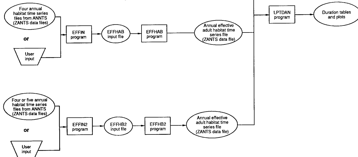
Fig. 9.1. Flow of information through the annual time series programs.
